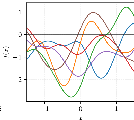
RBF GP prior realizations
