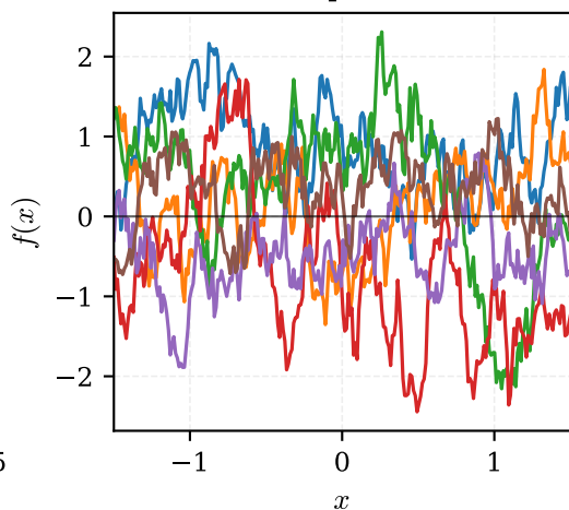
Matérn 1/2 GP prior realizations
