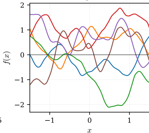
Matérn 5/2 GP prior realizations
