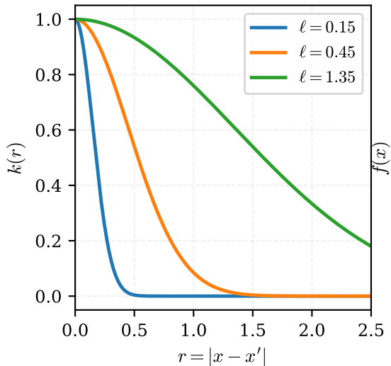
RBF kernel for varying \ell
