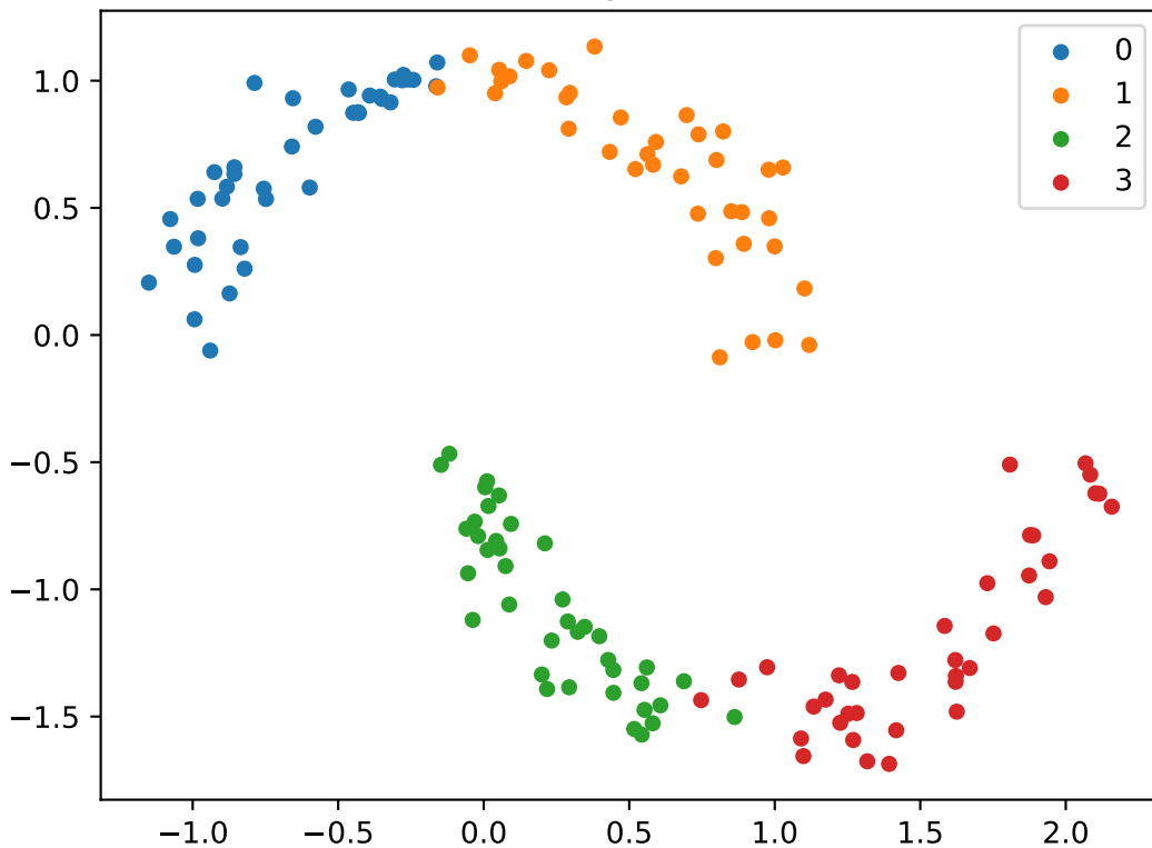
DPMC clustering on moon dataset
