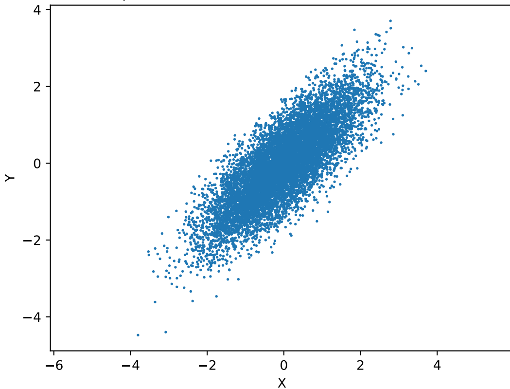
Samples from 2D Multivariate Normal Distribution
