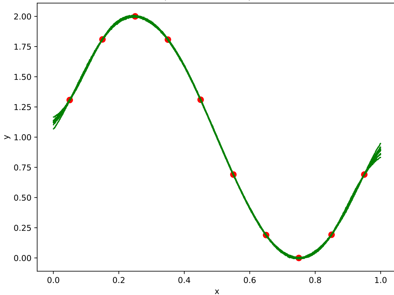
Samples from the GP posterior
