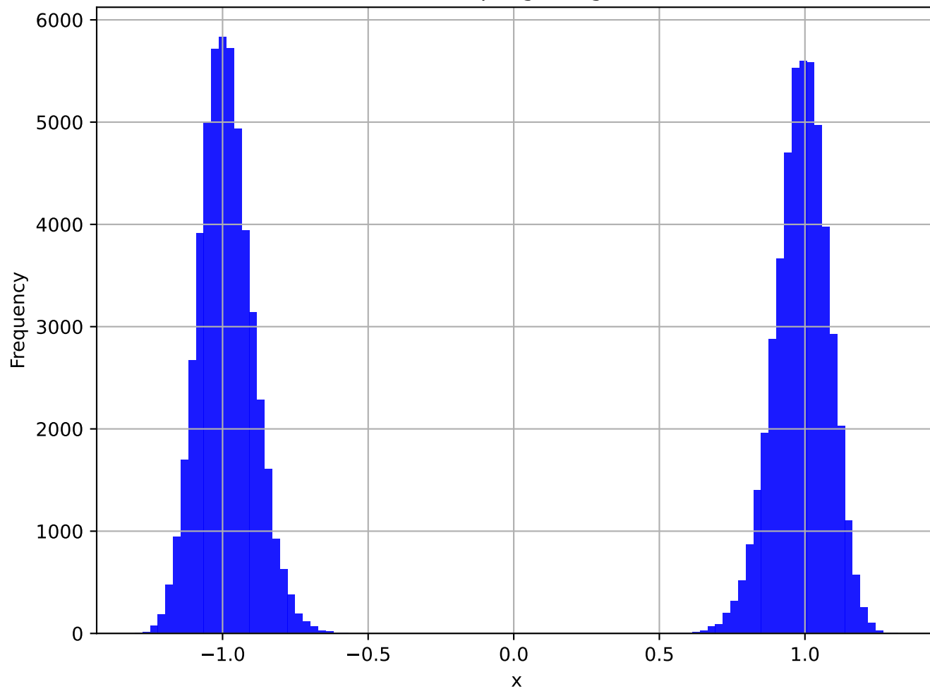
MCMC sampling using DRAM
