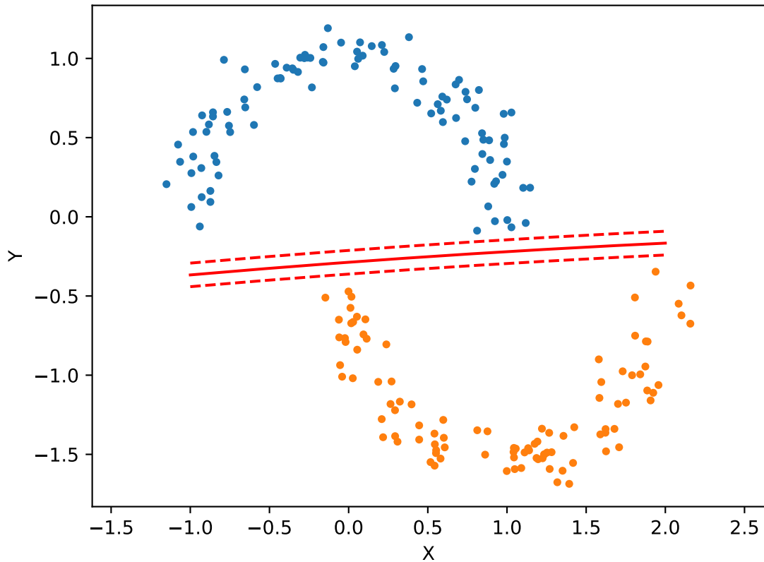
Naive Bayes Classifier Decision Boundary
