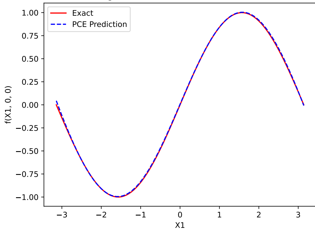
Ishigami Function Slice at X_2=0 , X_3=0
