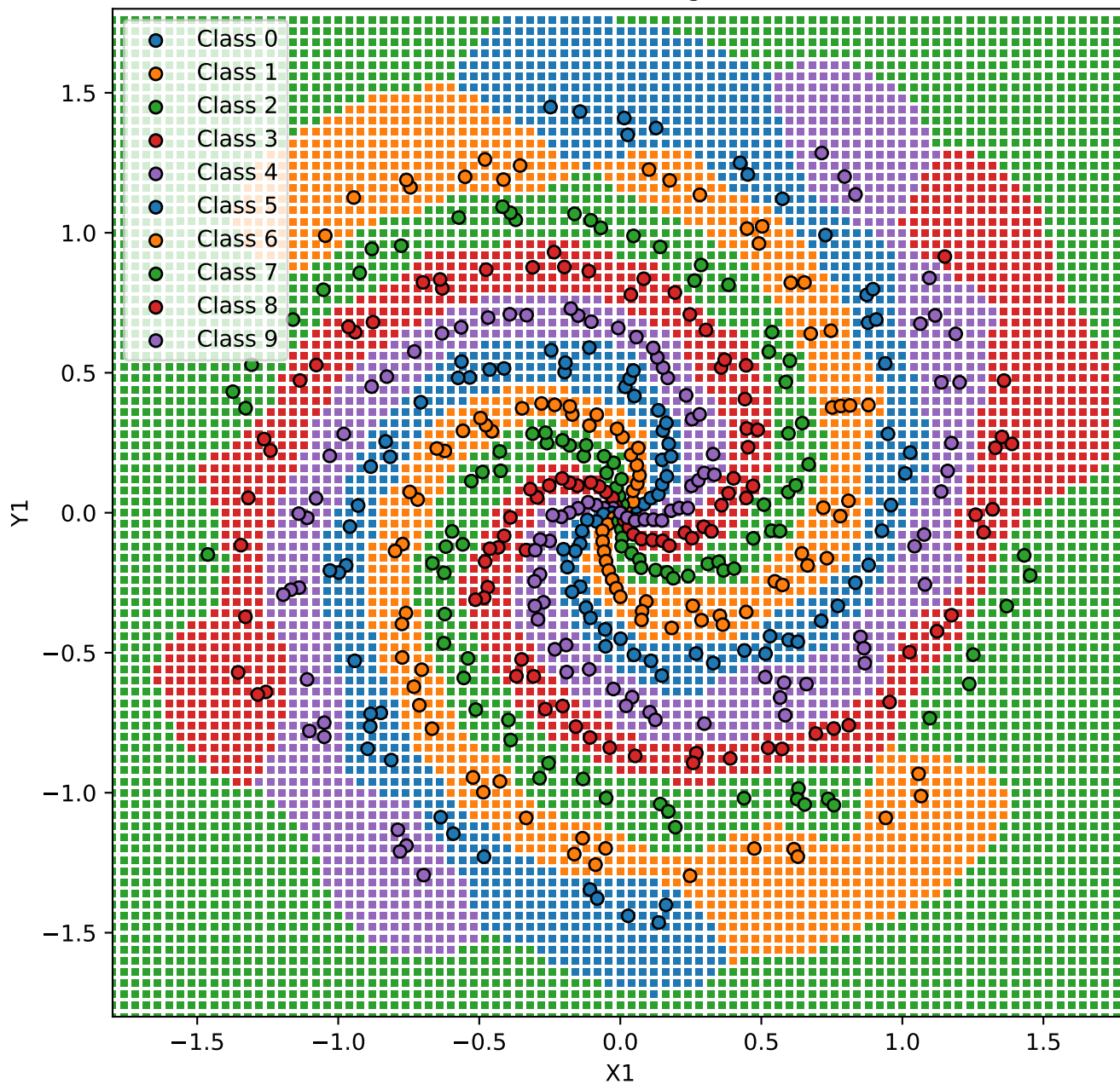
SVM Multi-class Decision Regions (10 Classes)
