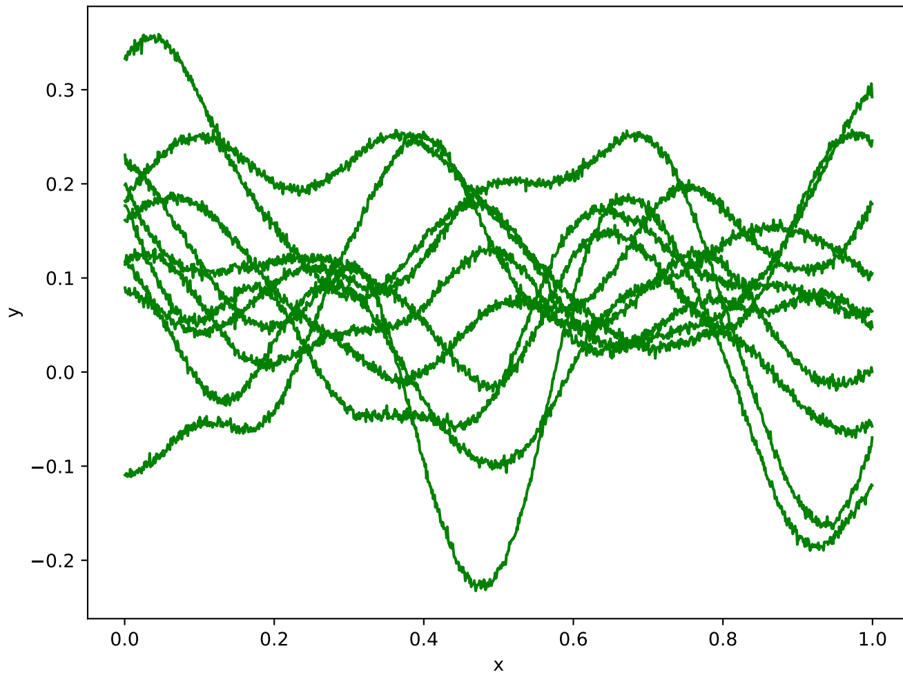
Samples from the GP prior
