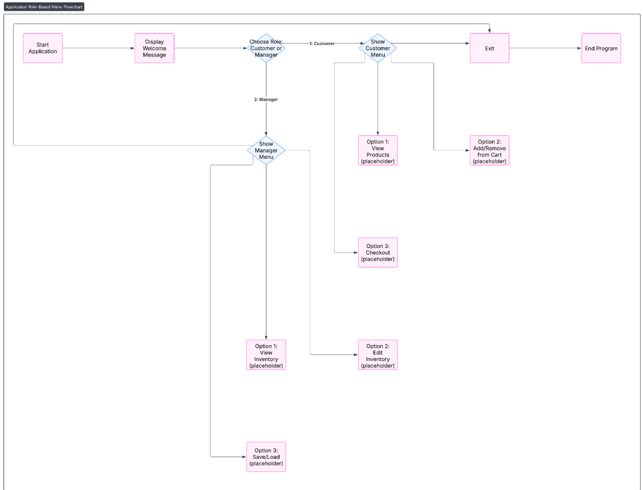
Figure 2 Program Flowchart
