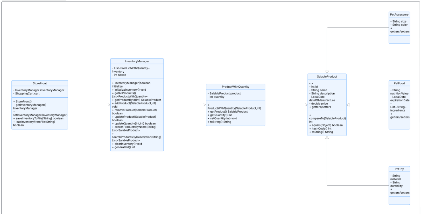
Figure 1 UML Diagram
