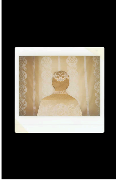
(02)
