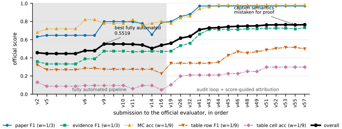
Figure 2: Official evaluator score for the 29 scored submissions we hold evaluator records for, in order. Ticks are labelled on a run’s first appearance; unlabelled ticks are re-uploads of an identical file, and one run has no surviving local prediction file. The shaded region is the fully automated pipeline; from v19 onwards every submission involves per-question intervention. The two components weighted 1/3 account for most of the movement, while the two table components weighted 1/9 stall between 0.05 and 0.52 and hold most of our remaining headroom. v55 regressed: we had labelled a caption-semantics inference “confirmed” when it was a heuristic, and reverting it returned exactly the +1.0 of evidence sum the arithmetic predicted. Drawn from results/official_scores.csv , which is built from the evaluator’s submission log.
