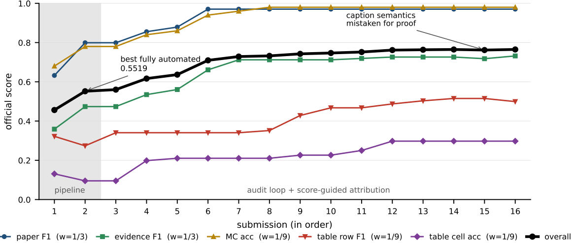
Figure 1: Official evaluator score for each of our sixteen scored submissions, in submission order. The shaded region is the pipeline; everything after it is the audit loop and score-guided attribution. The two components weighted 1/3 (paper F1, evidence F1) account for almost all of the movement, while the two table components weighted 1/9 stall around 0.30–0.50 and hold most of our remaining headroom. Submission 15 is the one that regressed: we had labelled a caption-semantics inference “confirmed” when it was a heuristic, and reverting it returned exactly the +1.0 of evidence sum the arithmetic predicted.
