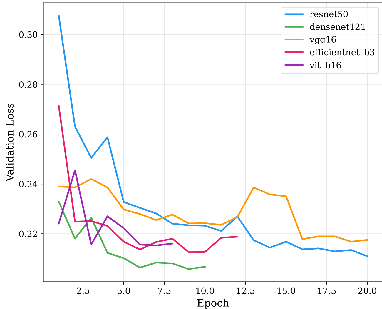
Validation Loss Curves
