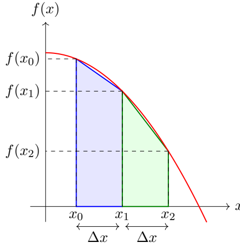
Figure 6: Illustration of the trapezoidal rule for numerical integration. The integral under the curve is approximated as a sum of trapezoidal areas.
