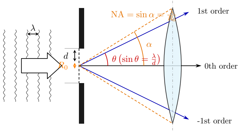
Figure 5: Smallest resolvable feature R_0 = \lambda/NA for a lens of numerical aperture NA = \sin \alpha , obtained by requiring the first diffraction order to fall within the acceptance cone.
