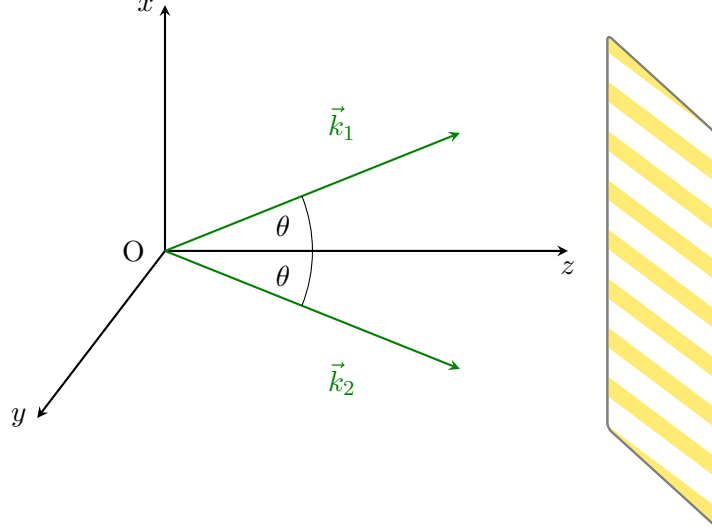
Figure 3: Interference of two plane waves propagating symmetrically with an angle 2\theta , creating an interference pattern on the screen (shown for \phi = 0 ).
