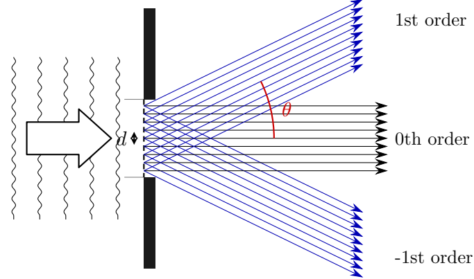
Figure 12: A feature of size d diffracts the probe beam into orders separated by \sin \theta = \lambda/d . Only orders within the lens acceptance angle are collected.
