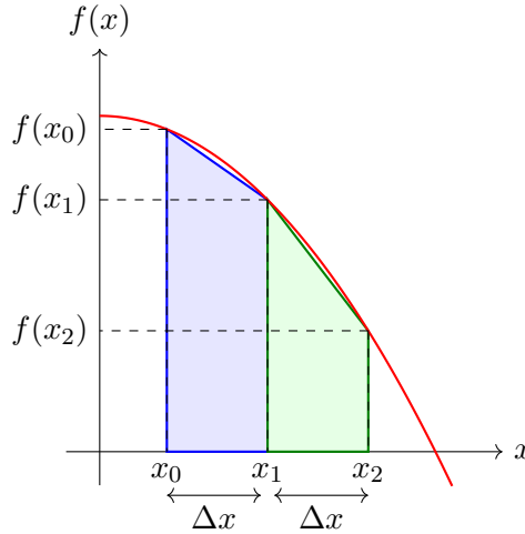
Figure 26: Illustration of the trapezoidal rule for numerical integration. The integral under the curve is approximated as a sum of trapezoidal areas.
