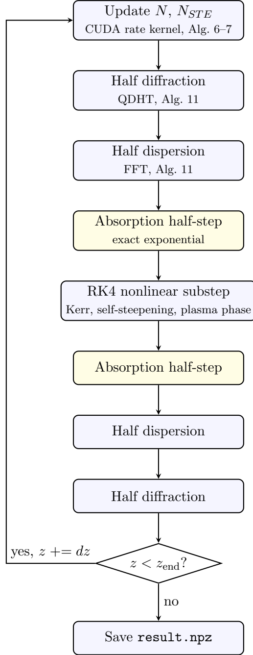
Figure 21: One iteration of the main propagation loop in Integrator.propagate . Every z step first advances the carrier populations along the full time axis at fixed r (Section 13), then applies the symmetric Strang sequence of diffraction, dispersion, and nonlinear substeps derived above to the field envelope. Diagnostics are recorded every save_stride steps (omitted here for clarity) before the loop repeats until z reaches the end of the propagation window.
