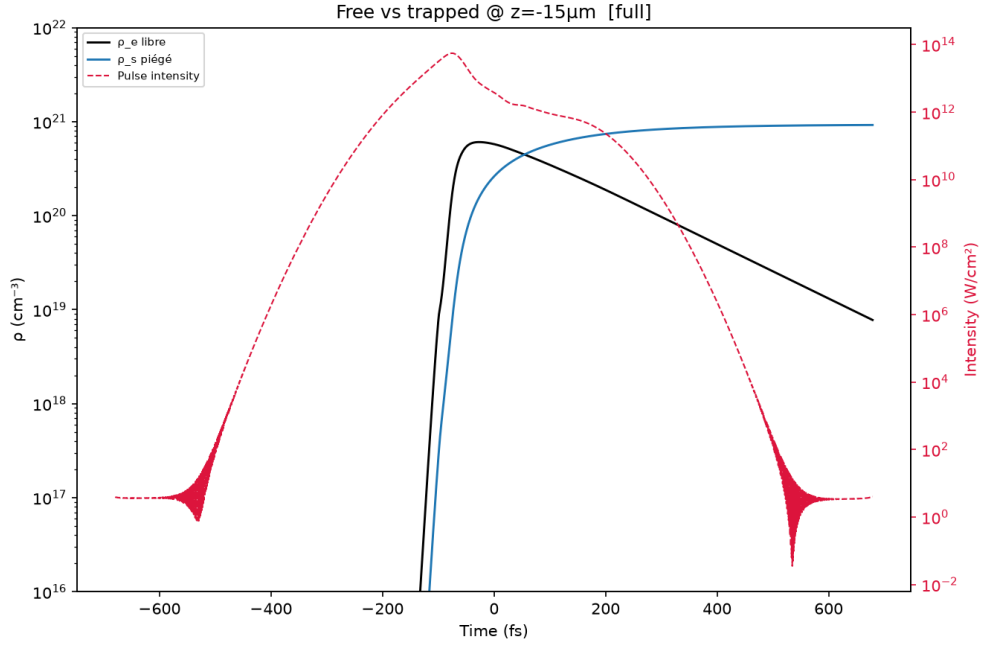
Figure 17: Free electron density N (black, labeled \rho_e libre) and trapped self-trapped exciton density N_{STE} (blue, labeled \rho_s piégé) on-axis at the nonlinear focus, against the local pulse intensity (dashed red). N rises together with the pulse and peaks close to the intensity maximum, then decays as electrons leave the conduction band through the trapping term N/\tau_r of the rate equations in Section 11.2. N_{STE} lags behind, rising as N is depleted and saturating once trapping is essentially complete, the microscopic bond-breaking process of Fig. 16 converting the transient free-carrier population into the permanent structural modification discussed above.
