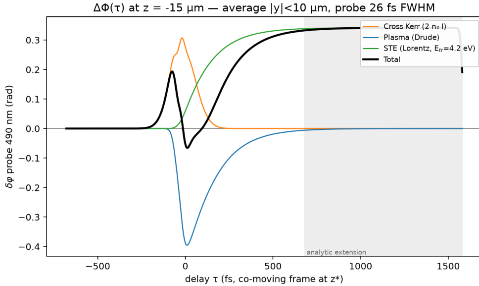
Figure 27: Predicted probe phase shift \delta\varphi(\tau) at 490 nm at the nonlinear focus, decomposed into its three channels (cross-Kerr, Drude plasma, bound STE) and their sum, convolved with a 26 fs probe pulse. The sequence reproduces the qualitative structure reported by Mouskettaras et al. [1] for single-pulse pump-probe interferometry in SiO 2 : an initial positive Kerr phase synchronous with the pump, an abrupt swing to negative as free carriers appear, and a delayed recovery to a positive plateau as trapping converts N into N_{STE} . The comparable magnitude of the Kerr and plasma contributions here, rather than Kerr dominating as in that reference, is expected given the different regime: this trace is taken at the filamentation clamping intensity, where n_2 I \approx N/(2\rho_c) by construction (Section 8.1), whereas the cited measurement was made well below threshold.
