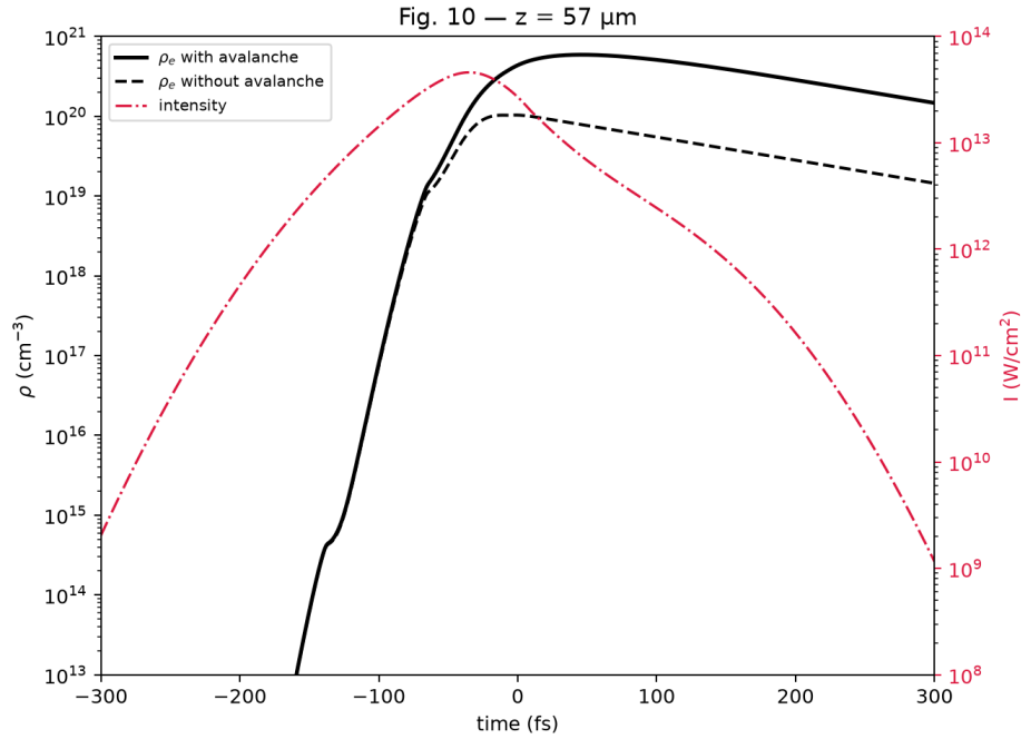
Figure 4: On-axis electron density at fixed z = 57 \mu\text{m} with and without the avalanche term \sigma_{\omega} I N / U_i of Eq. (38), reproducing Fig. 10 of [7] at 1.1 \mu\text{J} , 800 \text{ nm} . Photoionization alone (dashed) already produces a plateau once the pulse has passed, but avalanche multiplication (solid) drives the final density roughly a factor of six higher, showing that impact ionization contributes substantially to the total carrier yield once seeded by the multiphoton channel, even for the \sim 100 \text{ fs} pulse duration used here.
