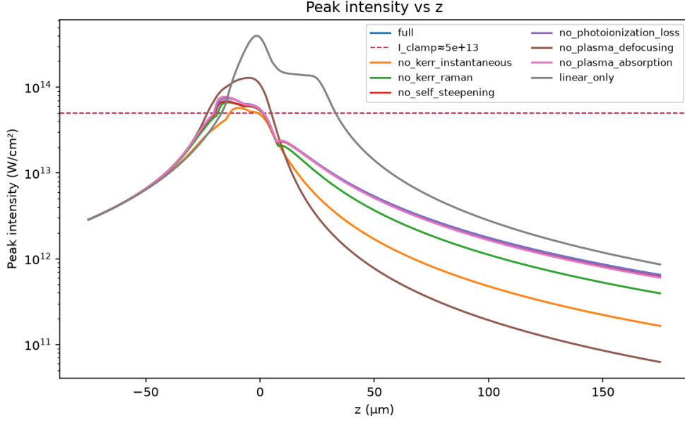
Figure 13: Peak on-axis intensity along z for the same conditions as Figs. 7b and 8 (800 nm, 160 fs, 1.1 \mu\text{J} ), this time with the self-trapped exciton channel active, and with each physical term of Eq. (38) disabled in turn. linear_only (pure diffraction and dispersion, no Kerr, no plasma) overshoots the clamping intensity by nearly an order of magnitude, confirming that the balance discussed in Section 8.1 is what limits the intensity in every other curve. no_plasma_defocusing keeps the ionization losses but removes the defocusing phase, and reaches roughly twice the clamping intensity before the accumulated photoionization and avalanche losses alone eventually arrest it, showing that defocusing, not absorption, does most of the clamping work. no_kerr_instantaneous and no_kerr_raman both peak lower than full and decay markedly faster past the nonlinear focus, roughly an order of magnitude below full by z = 150 \mu\text{m} , consistent with the weaker Kerr response lengthening L_c of Eq. (32). The remaining curves (no self-steepening, no photoionization loss, no plasma absorption) are visually indistinguishable from full at this scale, since none of them changes the dominant balance between Kerr self-focusing and plasma defocusing that sets the clamping intensity itself.
