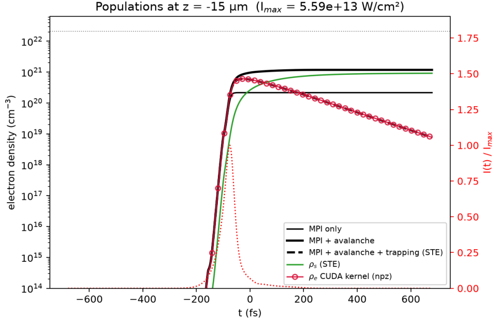
Figure 18: On-axis electron populations at the nonlinear focus for the 800 nm, 1.1 \mu\text{J} experiment of Fig. 8, reintegrating the 0D rate equations above from the saved intensity trace I(t) under three models (MPI only, +avalanche, +avalanche+trapping) and superposing the actual N(t) the CUDA kernel computed on-axis (open circles). The full model coincides with the CUDA output by construction, which is what this overlay is meant to check, and the agreement confirms the exponential-integrator time stepping of Section 12 reproduces the same rate equations solved here analytically term by term. Trapping into N_{STE} (green) becomes the dominant channel within a few hundred femtoseconds of the pulse peak, draining N (dashed black) down from its avalanche-augmented maximum, consistent with the trapping time \tau_r used throughout this report.
