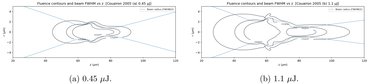
Figure 7: Fluence contours (solid black, in \text{J}/\text{cm}^2 ) and beam radius at half maximum (dashed blue) along the propagation axis, reproducing Fig. 7 of [7] at 800 nm, 160 fs, for two input pulse energies. At 0.45 \mu\text{J} the beam radius pinches once around the nonlinear focus and re-expands, the single self-focusing/defocusing cycle of Fig. 6. At 1.1 \mu\text{J} , above threshold by a larger margin, the pinch splits into two separate foci with a secondary local waist further downstream, a second refocusing cycle fed by the surrounding energy reservoir, consistent with the multiple-cycle picture of Section 1.3.12 of the Couairon review.
