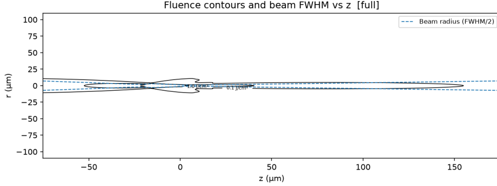
Figure 9: Fluence contours for the same 800\text{ nm} , 1.1\text{ }\mu\text{J} beam as Figure 7b, plotted over the full simulation box rather than zoomed on the nonlinear focus. Two things are visible that a single collapse would not produce. First, the 1.0\text{ J/cm}^2 contour is not a single smooth pinch between z \approx -30 and +10\text{ }\mu\text{m} : it wiggles, closing and reopening several times over that short stretch, each wiggle a candidate refocusing event happening too close to the previous one to be resolved as a separate, clean cycle at this scale. Second, the beam radius (dashed blue) starts narrowing again near the far edge of the box, past z \approx 130\text{ }\mu\text{m} , an incipient second cycle that the box is simply too short to complete. Both are evidence that the refocusing cycle described above is present in this run, not that it is well resolved by it.
