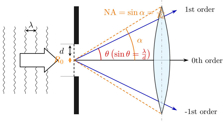
Figure 25: Smallest resolvable feature R_0 = \lambda/NA for a lens of numerical aperture NA = \sin \alpha , obtained by requiring the first diffraction order to fall within the acceptance cone.
