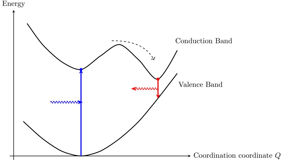
Figure 15: Configuration-coordinate diagram illustrating the formation of a self-trapped exciton (STE). After photoexcitation, a free exciton relaxes non-radiatively through lattice distortion into the STE configuration before radiative recombination.
