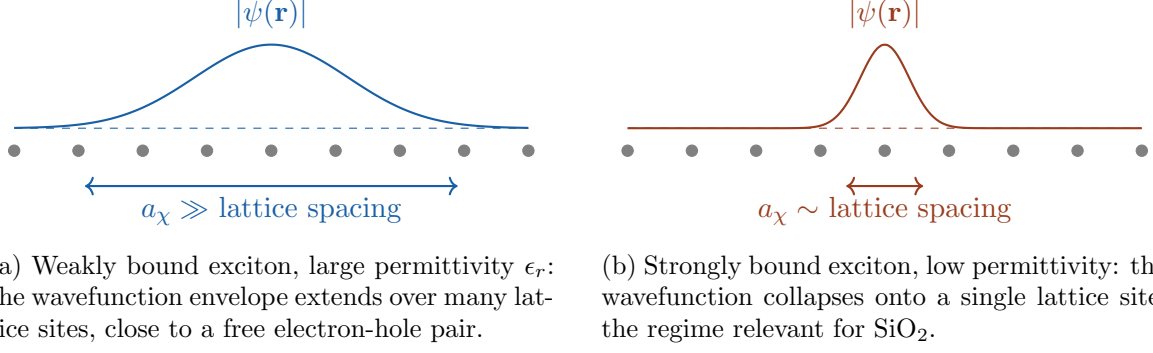
Figure 14: Spatial extent of the exciton wavefunction relative to the lattice spacing. The grey dots represent lattice atoms along one direction, the colored curve the envelope |\psi(\mathbf{r})| of the relative electron-hole wavefunction. A smaller \epsilon_r shrinks a_\chi from Eq. (37) until it reaches the strongly bound regime on the right.
