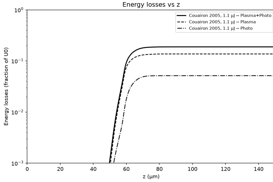
Figure 12: Cumulative energy lost by the pulse of [7] (at 1.1 \mu\text{J} ) as it propagates, as a fraction of the input energy U_0 , separated into the plasma absorption and photoionization channels. Both losses turn on together at the nonlinear focus and saturate once the beam has defocused past the clamping intensity, plasma absorption (inverse bremsstrahlung on already-free carriers) accounting for roughly 2.5\times more of the total loss than direct photoionization, consistent with the two channels' relative weight, \sigma_\omega/U_i against W_{PI}/\rho_{at} , discussed in Section 4.
