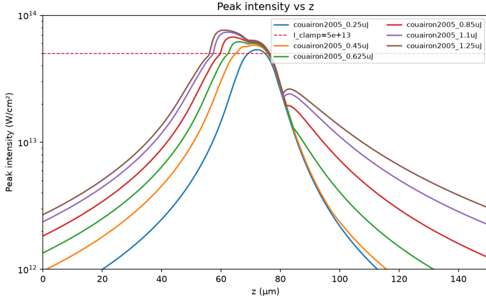
Figure 8: Peak on-axis intensity along z for six input pulse energies from 0.25 to 1.25 \mu\text{J} , reproducing Fig. 8 of [7]. Every curve rises together while the beam is still only linearly focusing, then the above-threshold curves ( P_{in} > P_{cr} , all but the lowest, 0.25 \mu\text{J} ) bend away from that common rise and saturate near the clamping intensity I_{clamp} \approx 5 \times 10^{13} \text{ W/cm}^2 (dashed line), each at its own z position given by L_{c,f} of Eq. (33) as discussed above. Past that peak, at larger z (deeper into the medium, beyond the nonlinear focus), every curve decreases again as the beam, now defocused by the plasma it just generated, diffracts away from the axis faster than the reservoir can refill it within the length of this box.
