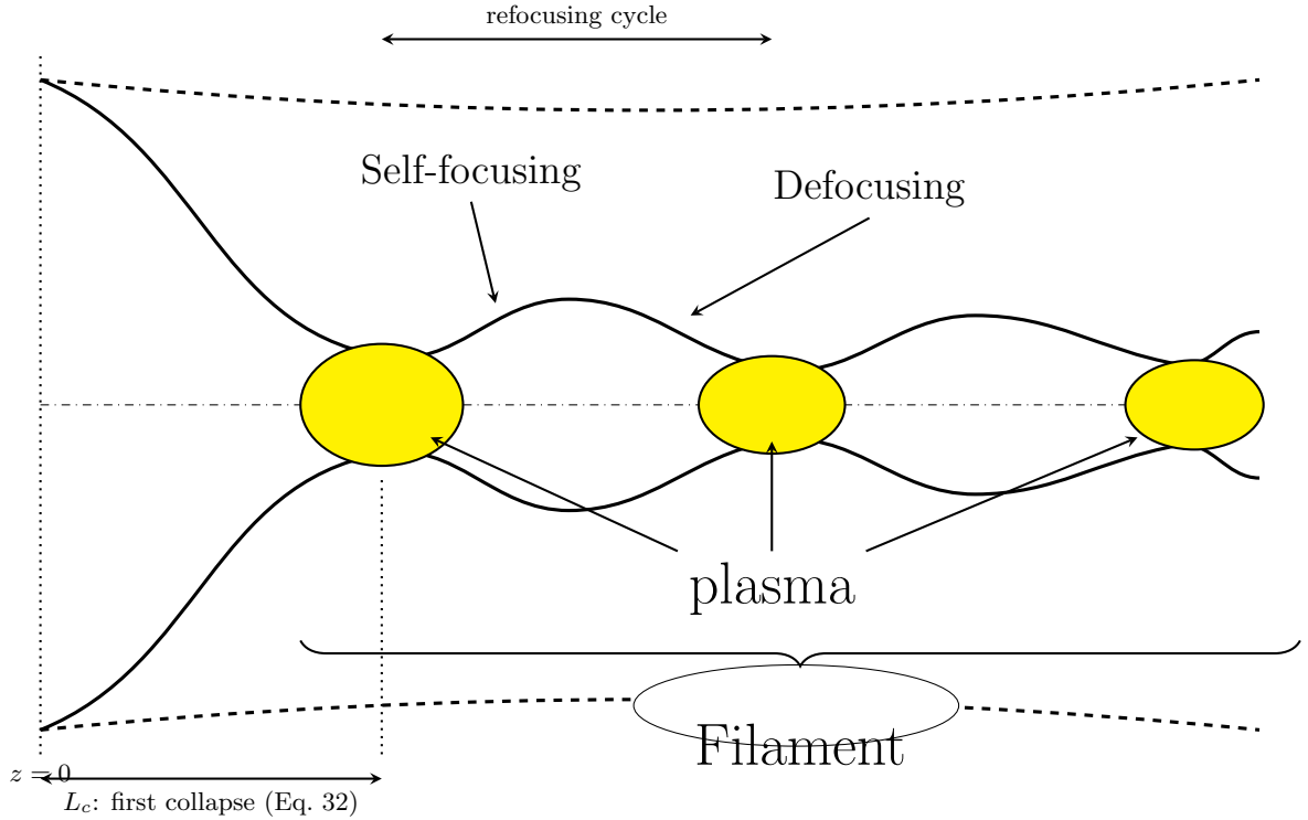
Figure 6: Schematic beam envelope undergoing repeated cycles of Kerr self-focusing and plasma defocusing, starting from an input beam launched at z = 0 . The first collapse occurs at z = L_c , given by Eq. (32). Each collapse is arrested before the beam reaches a singular focus by the free electron plasma generated near the intensity peak (yellow), which defocuses the beam until the intensity drops enough for the plasma to recombine and self-focusing to take back over, refilled by the surrounding energy reservoir. This repeated breathing over an extended propagation distance is the filament. Figure 9 shows this same sequence of collapses in an actual simulation, rather than as a schematic.
