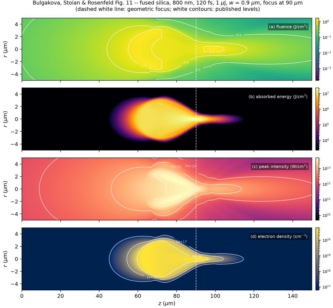
Figure 10: Fluence, absorbed energy density, peak intensity and electron density maps for the conditions of Bulgakova, Stoian & Rosenfeld (800 nm, 120 fs, 1 \mu\text{J} , w_0 = 0.9 \mu\text{m} , geometric focus at 90 \mu\text{m} below the surface, dashed white line), a parametrization independent of [7] (different n_2 , effective mass, collision time and lattice density). This is a second, independent instance of the same single collapse already seen in Figures 7 and 8, at different laser and material parameters, not a demonstration of multiple refocusing cycles (see Section 2.6.3 above for that). White contours mark the levels published in that reference; the solver's own fields (colour maps) fall within them across all four panels, including the secondary lobe past the geometric focus visible in panels (a)-(c), the start of a second cycle in the same sense as Figure 9.
