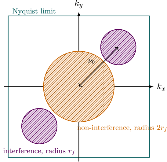
Figure 23: Layout of the interference orders in the Fourier plane of a recorded interferogram. The non-interference (zero order) blob of radius 2r_f sits at the origin, while the two interference sidebands of radius r_f sit at \pm\nu_0 along the carrier direction. Clean separation for filtering requires both sideband disks to stay outside the zero order disk and inside the square region the sensor can sample without aliasing, set by the Nyquist frequency \nu_N .
