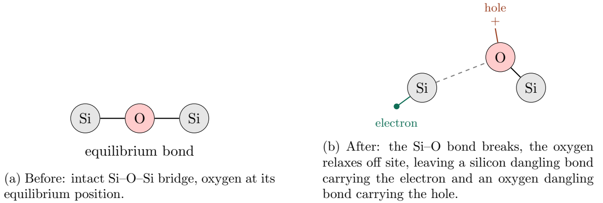
Figure 8: Schematic bond-breaking mechanism of self-trapping in \text{SiO}_2 , simplified to a linear Si–O–Si fragment for clarity (the real network is tetrahedrally coordinated). The two dangling bonds left behind are the microscopic identity of the self-trapped exciton.
