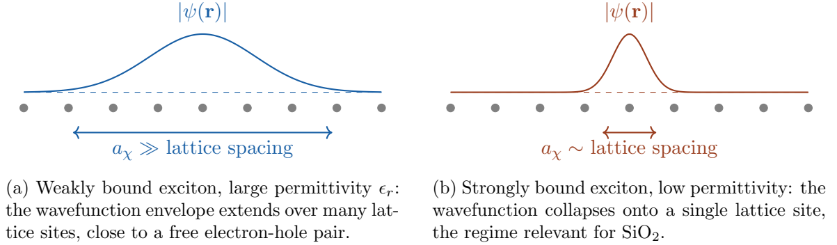
Figure 6: Spatial extent of the exciton wavefunction relative to the lattice spacing. The grey dots represent lattice atoms along one direction, the colored curve the envelope |\psi(\mathbf{r})| of the relative electron-hole wavefunction. A smaller \epsilon_r shrinks a_\chi from Eq. (37) until it reaches the strongly bound regime on the right.
