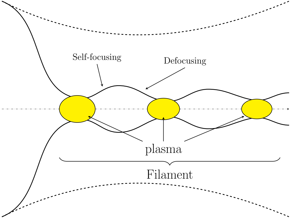
Figure 5: Schematic beam envelope (dashed outer curves: linear diffraction limit, solid inner curves: actual beam radius) undergoing repeated cycles of Kerr self-focusing and plasma defocusing. Each collapse is arrested before catastrophic self-focusing by the free electron plasma generated near the intensity peak (yellow), which defocuses the beam until the intensity drops enough for the plasma to recombine and self-focusing to take over again, refilled by the surrounding energy reservoir. This repeated breathing over an extended propagation distance is the filament.
