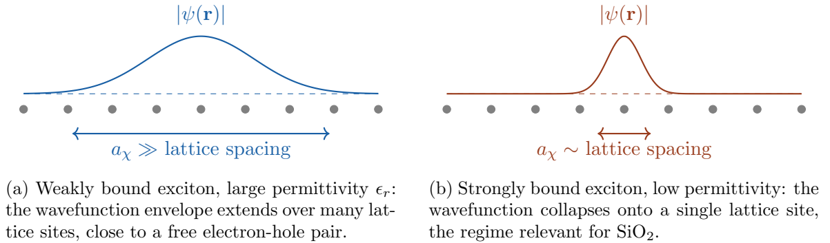
Figure 5: Spatial extent of the exciton wavefunction relative to the lattice spacing. The grey dots represent lattice atoms along one direction, the colored curve the envelope |\psi(\mathbf{r})| of the relative electron-hole wavefunction. A smaller \epsilon_r shrinks a_\chi from Eq. (37) until it reaches the strongly bound regime on the right.
