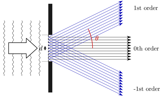
Figure 10: A feature of size d diffracts the probe beam into orders separated by \sin \theta = \lambda/d . Only orders within the lens acceptance angle are collected.
