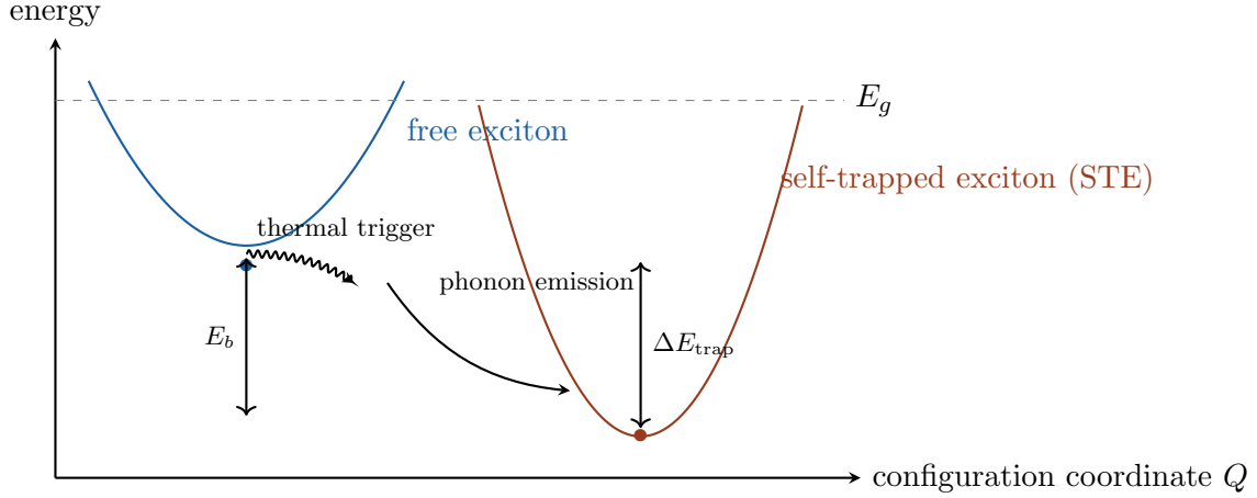
Figure 6: Configuration coordinate diagram for self-trapping. The free exciton sits in a shallow well close to the gap E_g . A thermal fluctuation displaces the lattice along Q , and once the exciton-phonon coupling is strong enough there is no barrier back to a much deeper, displaced well, the self-trapped exciton state. The energy difference \Delta E_{\text{trap}} between the two minima is released into local phonons.
