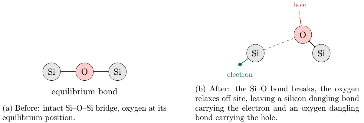
Figure 7: Schematic bond-breaking mechanism of self-trapping in \text{SiO}_2 , simplified to a linear Si–O–Si fragment for clarity (the real network is tetrahedrally coordinated). The two dangling bonds left behind are the microscopic identity of the self-trapped exciton.
