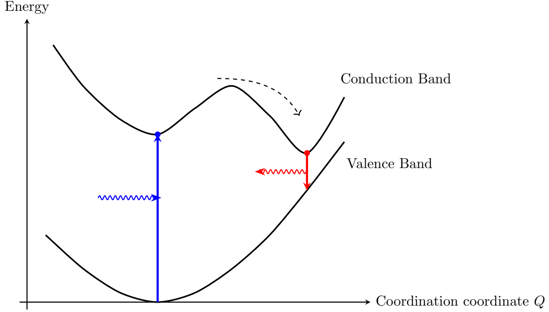
Figure 12: Configuration-coordinate diagram illustrating the formation of a self-trapped exciton (STE). After photoexcitation, a free exciton relaxes non-radiatively through lattice distortion into the STE configuration before radiative recombination.
