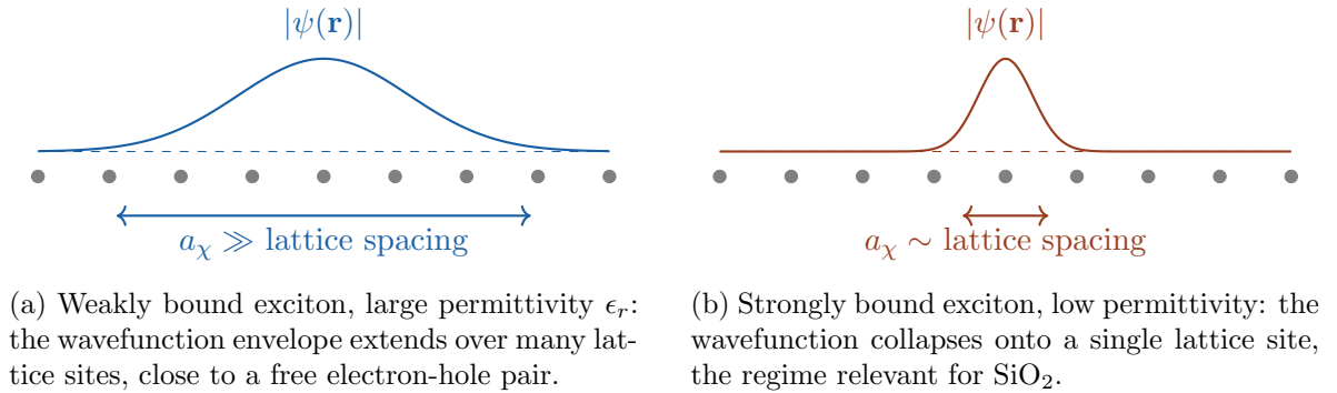
Figure 11: Spatial extent of the exciton wavefunction relative to the lattice spacing. The grey dots represent lattice atoms along one direction, the colored curve the envelope |\psi(\mathbf{r})| of the relative electron-hole wavefunction. A smaller \epsilon_r shrinks a_\chi from Eq. (33) until it reaches the strongly bound regime on the right.
