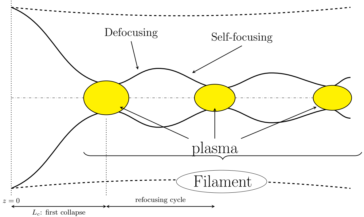
Figure 8: Schematic beam envelope undergoing repeated cycles of Kerr self-focusing and plasma defocusing, starting from an input beam launched at z = 0 . The first collapse occurs at z = L_c , the collapse length. Each collapse is arrested before the beam reaches a singular focus by the free electron plasma generated near the intensity peak (yellow), which defocuses the beam until the intensity drops enough for the plasma to recombine and self-focusing to take back over, refilled by the surrounding energy reservoir. This repeated breathing over an extended propagation distance is the filament.
