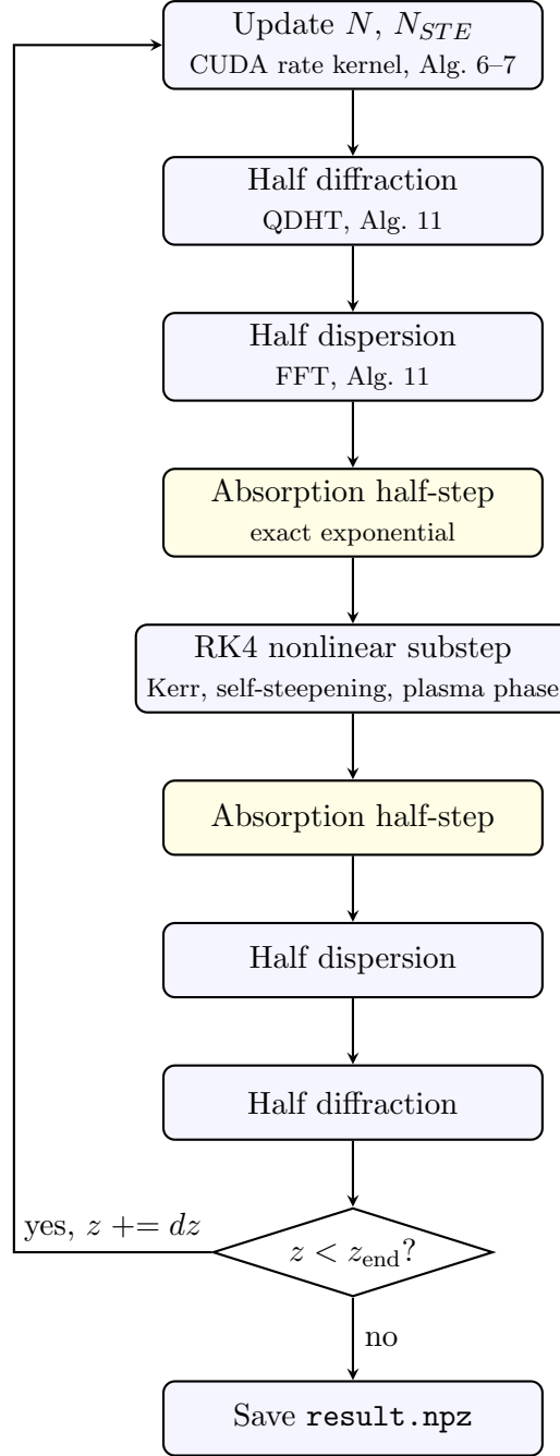
Figure 25: One iteration of the main propagation loop in Integrator.propagate . Every z step first advances the carrier populations along the full time axis at fixed r (Section 6), then applies the symmetric Strang sequence of diffraction, dispersion, and nonlinear substeps derived above to the field envelope. Diagnostics are recorded every save_stride steps (omitted here for clarity) before the loop repeats until z reaches the end of the propagation window.
