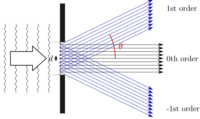
Figure 17: A feature of size d diffracts the probe beam into orders separated by \sin \theta = \lambda/d . Only orders within the lens acceptance angle are collected.
