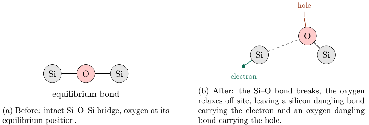
Figure 13: Schematic bond-breaking mechanism of self-trapping in SiO 2 , simplified to a linear Si–O–Si fragment for clarity (the real network is tetrahedrally coordinated). The two dangling bonds left behind are the microscopic identity of the self-trapped exciton.
