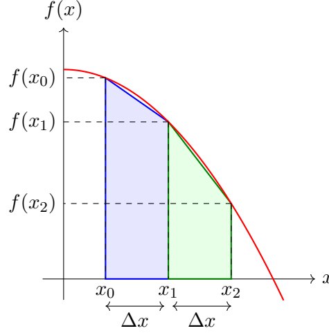
Figure 19: Illustration of the trapezoidal rule for numerical integration. The integral under the curve is approximated as a sum of trapezoidal areas.
