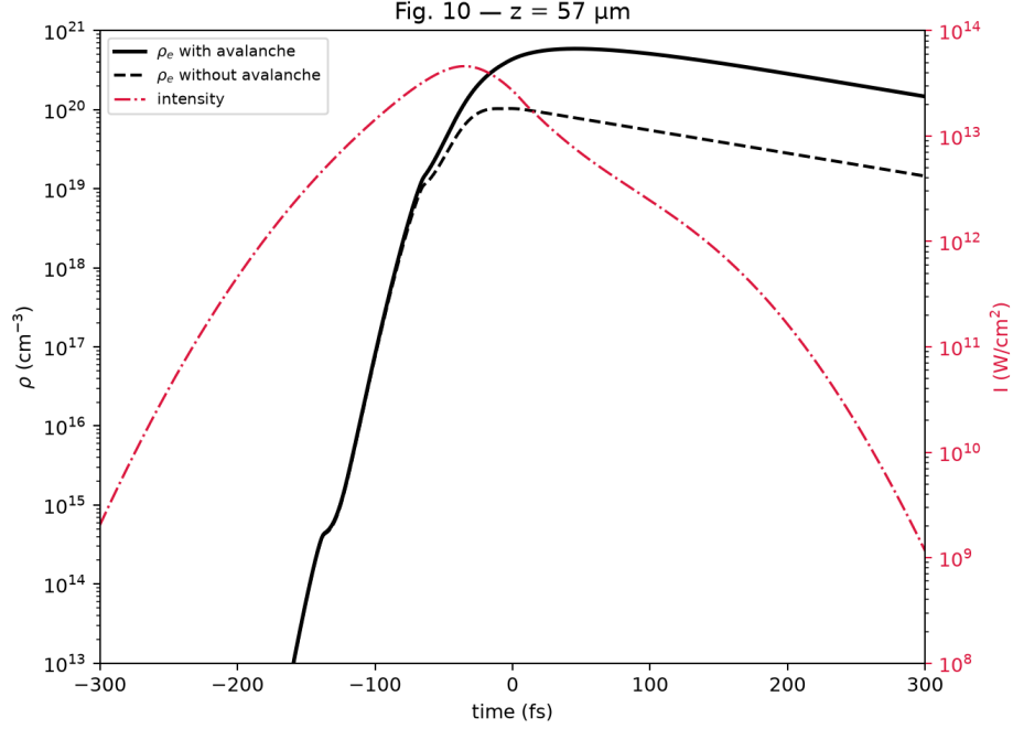
Figure 4: On-axis electron density at fixed z = 57 \mu\text{m} with and without the avalanche term \sigma_\omega I N/U_i of Eq. (51), reproducing Fig. 10 of [7] at 1.1 \mu\text{J} , 800 \text{ nm} . Photoionization alone (dashed) already produces a plateau once the pulse has passed, but avalanche multiplication (solid) drives the final density roughly a factor of six higher, showing that impact ionization contributes substantially to the total carrier yield once seeded by the multiphoton channel, even for the \sim 100 \text{ fs} pulse duration used here.
