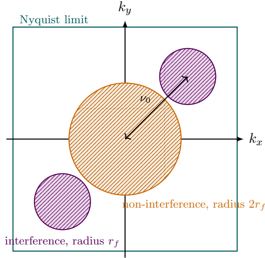
Figure 16: Layout of the interference orders in the Fourier plane of a recorded interferogram. The non-interference (zero order) blob of radius 2r_f sits at the origin, while the two interference sidebands of radius r_f sit at \pm\nu_0 along the carrier direction. Clean separation for filtering requires both sideband disks to stay outside the zero order disk and inside the square region the sensor can sample without aliasing, set by the Nyquist frequency \nu_N .
