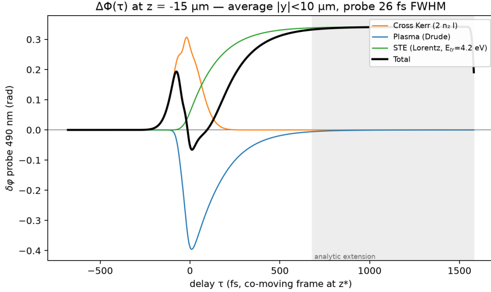
Figure 26: Predicted probe phase shift \delta\varphi(\tau) at 490 nm at the nonlinear focus, decomposed into its three channels (cross-Kerr, Drude plasma, bound STE) and their sum, convolved with a 26 fs probe pulse. The sequence reproduces the qualitative structure reported by Mouskeftaras et al. [1] for single-pulse pump-probe interferometry in SiO 2 : an initial positive Kerr phase synchronous with the pump, an abrupt swing to negative as free carriers appear, and a delayed recovery to a positive plateau as trapping converts N into N_{STE} . The comparable magnitude of the Kerr and plasma contributions here, rather than Kerr dominating as in that reference, is expected given the different regime: this trace is taken at the filamentation clamping intensity, where n_2 I \approx N/(2\rho_c) by construction (Section 2.6), whereas the cited measurement was made well below threshold.
