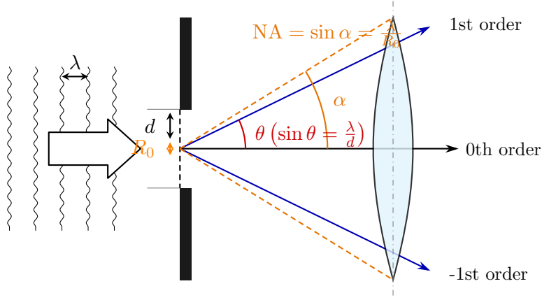
Figure 18: Smallest resolvable feature R_0 = \lambda/NA for a lens of numerical aperture NA = \sin \alpha , obtained by requiring the first diffraction order to fall within the acceptance cone.
