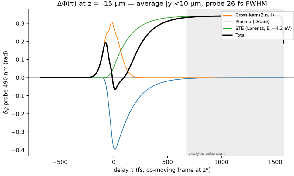
Figure 19: Predicted probe phase shift \delta\varphi(\tau) at 490 nm at the nonlinear focus, decomposed into its three channels (cross-Kerr, Drude plasma, bound STE) and their sum, convolved with a 26 fs probe pulse. The sequence reproduces the qualitative structure reported by Mouskettaras et al. [1] for single-pulse pump-probe interferometry in SiO 2 : an initial positive Kerr phase synchronous with the pump, an abrupt swing to negative as free carriers appear, and a delayed recovery to a positive plateau as trapping converts N into N_{STE} . The comparable magnitude of the Kerr and plasma contributions here, rather than Kerr dominating as in that reference, is expected given the different regime: this trace is taken at the filamentation clamping intensity, where n_2 I \approx N/(2\rho_c) by construction (Section 2.6), whereas the cited measurement was made well below threshold.
