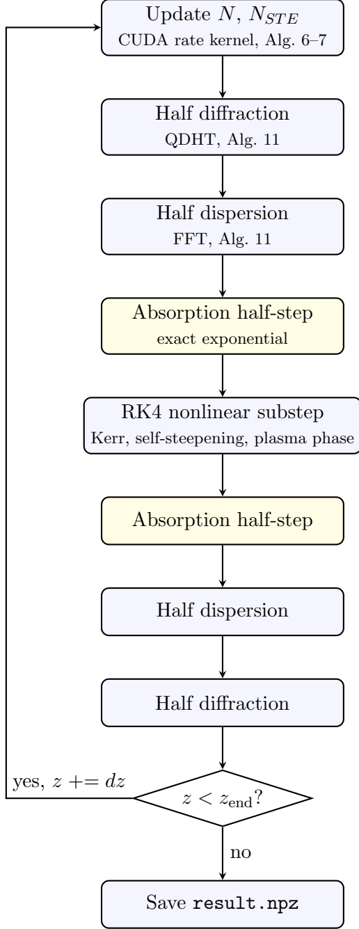
Figure 18: One iteration of the main propagation loop in Integrator.propagate . Every z step first advances the carrier populations along the full time axis at fixed r (Section 6), then applies the symmetric Strang sequence of diffraction, dispersion, and nonlinear substeps derived above to the field envelope. Diagnostics are recorded every save_stride steps (omitted here for clarity) before the loop repeats until z reaches the end of the propagation window.
