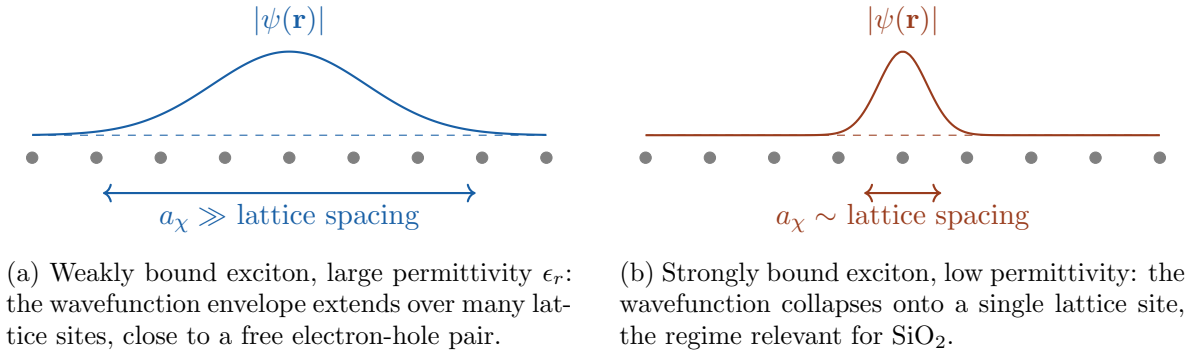
Figure 7: Spatial extent of the exciton wavefunction relative to the lattice spacing. The grey dots represent lattice atoms along one direction, the colored curve the envelope |\psi(\mathbf{r})| of the relative electron-hole wavefunction. A smaller \epsilon_r shrinks a_\chi from Eq. (33) until it reaches the strongly bound regime on the right.
