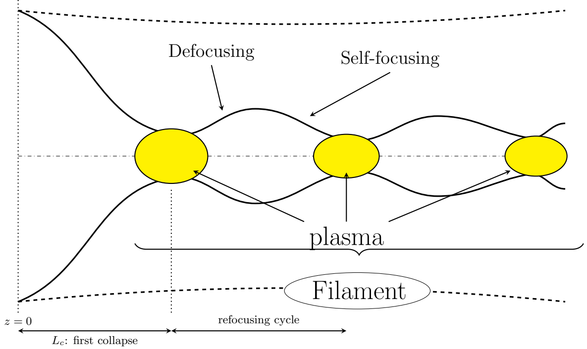
Figure 6: Schematic beam envelope undergoing repeated cycles of Kerr self-focusing and plasma defocusing, starting from an input beam launched at z = 0 . The first collapse occurs at z = L_c , the collapse length. Each collapse is arrested before the beam reaches a singular focus by the free electron plasma generated near the intensity peak (yellow), which defocuses the beam until the intensity drops enough for the plasma to recombine and self-focusing to take back over, refilled by the surrounding energy reservoir. This repeated breathing over an extended propagation distance is the filament.
