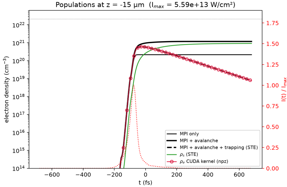
Figure 15: On-axis electron populations at the nonlinear focus for the 800 nm, 1.1 \mu\text{J} experiment, reintegrating the 0D rate equations above from the saved intensity trace I(t) under three models (MPI only, +avalanche, +avalanche+trapping) and superposing the actual N(t) the CUDA kernel computed on-axis (open circles). The full model coincides with the CUDA output by construction, which is what this overlay is meant to check, and the agreement confirms the exponential-integrator time stepping of Section 5 reproduces the same rate equations solved here analytically term by term. Trapping into N_{STE} (green) becomes the dominant channel within a few hundred femtoseconds of the pulse peak, draining N (dashed black) down from its avalanche-augmented maximum, consistent with the trapping time \tau_r used throughout this report.
