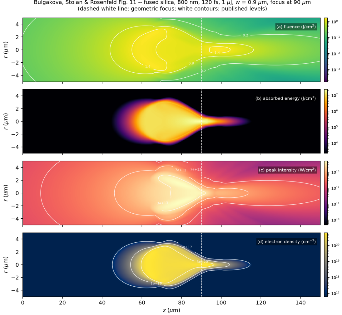
Figure 9: Fluence, absorbed energy density, peak intensity and electron density maps for the conditions of Bulgakova, Stoian & Rosenfeld (800 nm, 120 fs, 1 \mu\text{J} , w_0 = 0.9 \mu\text{m} , geometric focus at 90 \mu\text{m} below the surface, dashed white line), a parametrization independent of [7] (different n_2 , effective mass, collision time and lattice density). White contours mark the levels published in that reference; the solver's own fields (colour maps) fall within them across all four panels, including the secondary lobe past the geometric focus visible in panels (a)–(c), itself a signature of the refocusing cycle of Fig. 6.
