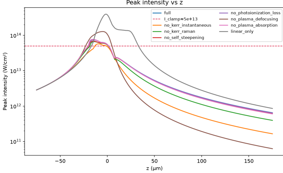
Figure 12: Peak on-axis intensity along z for the experiment actually used throughout this report (1030 nm, 263 fs, 15 \mu\text{J} , self-trapped exciton channel active), with each physical term of Eq. (37) disabled in turn. linear_only (pure diffraction and dispersion, no Kerr, no plasma) overshoots the clamping intensity by nearly an order of magnitude, confirming that the balance discussed in Section 8.1 is what limits the intensity in every other curve. no_plasma_defocusing keeps the ionization losses but removes the defocusing phase, and reaches roughly twice the clamping intensity before the accumulated photoionization and avalanche losses alone eventually arrest it, showing that defocusing, not absorption, does most of the clamping work. no_kerr_instantaneous and no_kerr_raman both peak lower than full and decay markedly faster past the nonlinear focus, roughly an order of magnitude below full by z = 150 \mu\text{m} , consistent with the weaker Kerr response lengthening L_c of Eq. (31). The remaining curves (no self-steepening, no photoionization loss, no plasma absorption) are visually indistinguishable from full at this scale, since none of them changes the dominant balance between Kerr self-focusing and plasma defocusing that sets the clamping intensity itself.
