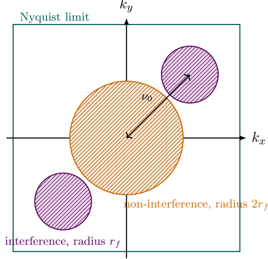
Figure 22: Layout of the interference orders in the Fourier plane of a recorded interferogram. The non-interference (zero order) blob of radius 2r_f sits at the origin, while the two interference sidebands of radius r_f sit at \pm\nu_0 along the carrier direction. Clean separation for filtering requires both sideband disks to stay outside the zero order disk and inside the square region the sensor can sample without aliasing, set by the Nyquist frequency \nu_N .
