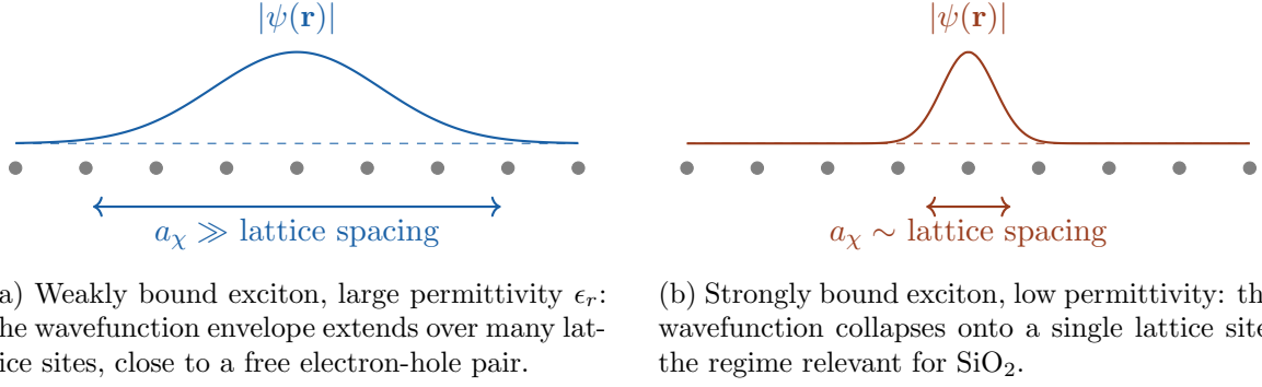
Figure 13: Spatial extent of the exciton wavefunction relative to the lattice spacing. The grey dots represent lattice atoms along one direction, the colored curve the envelope |\psi(\mathbf{r})| of the relative electron-hole wavefunction. A smaller \epsilon_r shrinks a_\chi from Eq. (36) until it reaches the strongly bound regime on the right.
