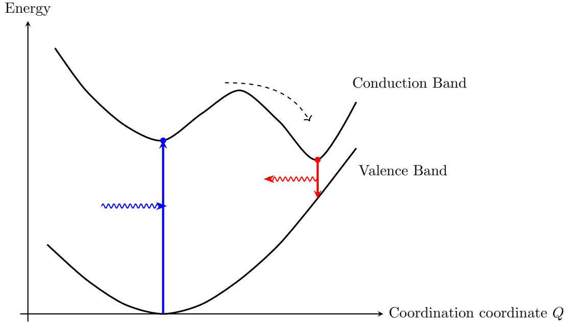
Figure 14: Configuration-coordinate diagram illustrating the formation of a self-trapped exciton (STE). After photoexcitation, a free exciton relaxes non-radiatively through lattice distortion into the STE configuration before radiative recombination.
