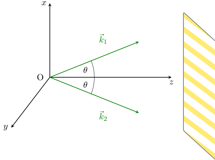
Figure 21: Interference of two plane waves propagating symmetrically with an angle 2\theta , creating an interference pattern on the screen (shown for \phi = 0 ).
