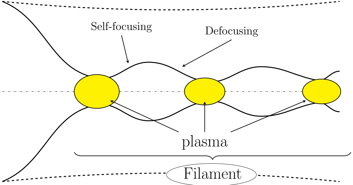
Figure 6: Schematic beam envelope undergoing repeated cycles of Kerr self-focusing and plasma defocusing. Each collapse is arrested before catastrophic self-focusing by the free electron plasma generated near the intensity peak (yellow), which defocuses the beam until the intensity drops enough for the plasma to recombine and self-focusing to take over again, refilled by the surrounding energy reservoir. This repeated breathing over an extended propagation distance is the filament.
