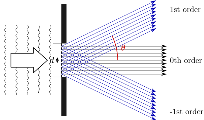
Figure 23: A feature of size d diffracts the probe beam into orders separated by \sin \theta = \lambda/d . Only orders within the lens acceptance angle are collected.
