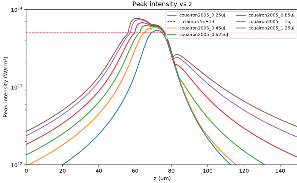
Figure 8: Peak on-axis intensity along z for six input pulse energies from 0.25 to 1.25 \mu\text{J} , reproducing Fig. 8 of [7]. Below threshold the peak intensity simply follows linear focusing (lower curves never reach I_{\text{clamp}} ). Above it, every curve saturates at essentially the same value close to the clamping intensity I_{\text{clamp}} \approx 5 \times 10^{13} \text{ W}/\text{cm}^2 (dashed line) predicted from the intensity-clamping balance of Section 1.3.4 of the Couairon notes, before decaying on the trailing side of the nonlinear focus. This saturation, common to all above-threshold energies despite their different P_{\text{in}}/P_{\text{cr}} ratios, is the numerical signature of intensity clamping referred to throughout Section 8.2.
