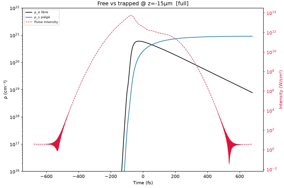
Figure 16: Free electron density N (black, labeled \rho_e libre) and trapped self-trapped exciton density N_{STE} (blue, labeled \rho_s piégé) on-axis at the nonlinear focus, against the local pulse intensity (dashed red). N rises together with the pulse and peaks close to the intensity maximum, then decays as electrons leave the conduction band through the trapping term N/\tau_r of the rate equations in Section 11.2. N_{STE} lags behind, rising as N is depleted and saturating once trapping is essentially complete, the microscopic bond-breaking process of Fig. 15 converting the transient free-carrier population into the permanent structural modification discussed above.
