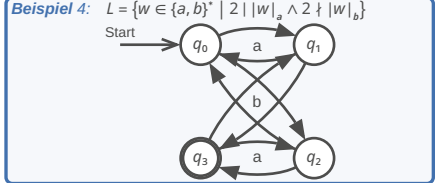
Beispiel 4: L = \{w \in \{a, b\}^* \mid 2 \mid |w|_a \wedge 2 \nmid |w|_b\}
