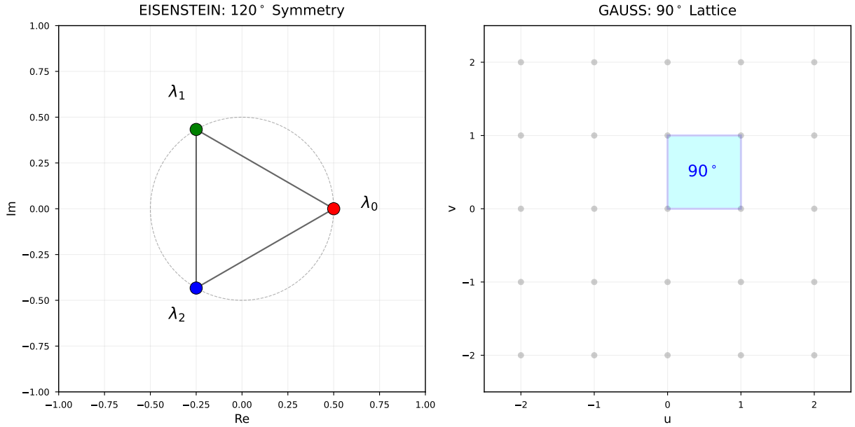
Figure 3. Gauss–Eisenstein duality mediated by \varphi . Left: The tripartite operator \hat{\Omega} with eigenvalues \lambda_k = \frac{1}{2}\omega^k separated by 120^\circ (Eisenstein structure). Right: The rectangular lattice \Lambda_{\text{PCF}} = \mathbb{Z}M \oplus \mathbb{Z}Mi with 90^\circ fundamental cell (Gauss structure). The arrow “PCF \rightarrow ” denotes the transformation chain: Eisenstein ( 120^\circ ) \rightarrow scalar periodicity \rightarrow Gauss ( 90^\circ ). Golden mediation preserves the invariant |\Omega| = 1/2 while effecting the symmetry transition S_3 \rightarrow \mathbb{Z}_4 , generating the spectral parameters \mu = 1/2, \sigma = 3\mu = 3/2 .
