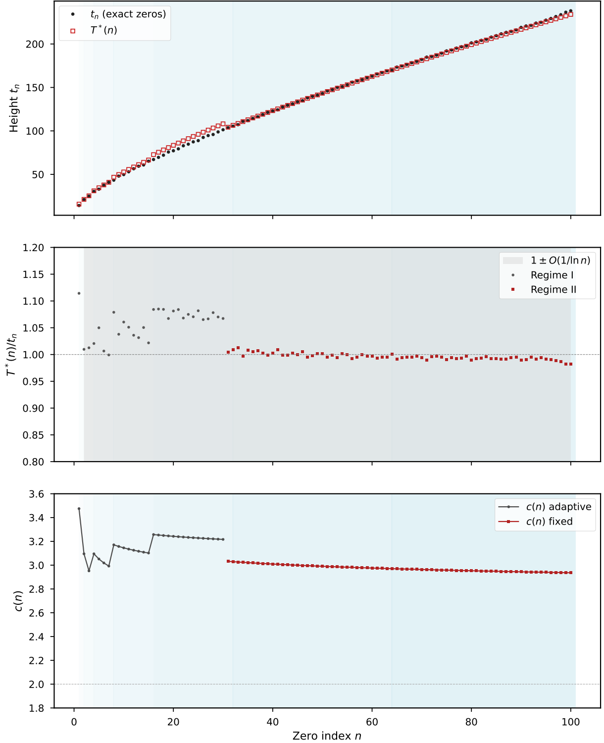
Figure 9. Dual spectral structure of T^* . (a) Zero heights t_n (filled) vs. T^*(n) (open squares), n = 1, \dots, 100 . Bands: hypercube generations G_k = [2^k, 2^{k+1}) ; dotted lines: Mersenne primes M_2=3 , M_3=7 , M_5=31 ; dashed line at n=30 : Regime I/II boundary. (b) Ratio T^*(n)/t_n : Regime I (gray) oscillates; Regime II (red) follows the peaked structure of Theorem 4.2. (c) Modulation c(n, \alpha, \beta) : adaptive (Regime I) with discontinuities at 2^k ; fixed (Regime II) decaying toward \sigma + \mu = 2 .
