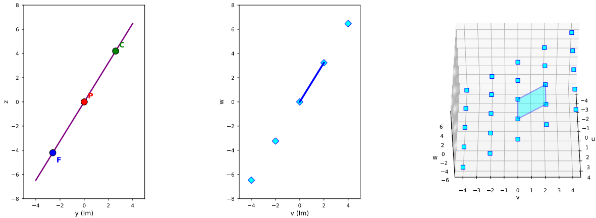
Figure 6. Golden mediation between Eisenstein and Gauss structures (III: Lateral and isometric views). Projective views revealing structural constraints. Left: Vertices aligned on z = \varphi y . Center: Lattice cell degenerating on w = \varphi v . Right: Isometric view showing the fundamental cell as a rhombus. The golden ratio \varphi unifies both structures, preserving |\Omega| = 1/2 throughout.
