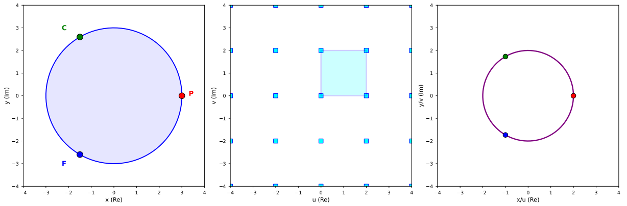
Figure 5. Golden mediation between Eisenstein and Gauss structures (II: Top views). Planar projections of the correspondence. Left: Circle R_0 = 3 with inscribed 120^\circ triangle (Eisenstein structure). Center: Square cell M_{\text{PCF}} \times M_{\text{PCF}} (Gauss structure). Right: Superposition of circle-plus-triangle within square.
