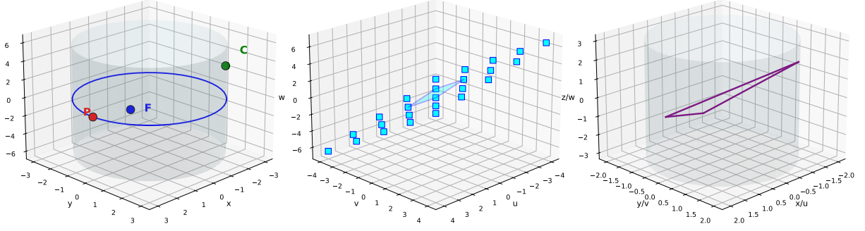
Figure 4. Golden mediation between Eisenstein and Gauss structures (I: 3D views). Three-dimensional views of the cylinder–lattice correspondence through the coupling z = \varphi y . Left: Cylinder C_0 with equilateral triangle P - C - F . Center: Lattice \Lambda_{\text{PCF}} with parallelogram fundamental cell. Right: Superposition showing the triangle embedded in the lattice.
