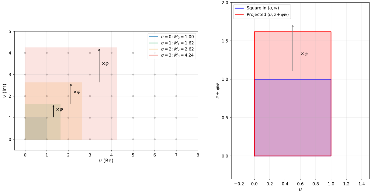
Figure 7. PCF pentadimensional lattice tower with \varphi^\sigma scaling (I). Top left: Lattice \Lambda_{\text{PCF}} with fundamental cells M_\sigma = M_{\text{PCF}} \cdot \varphi^\sigma at levels \sigma = 0, 1, 2, 3 , showing self-similar growth by factor \varphi between consecutive levels. Top right: Golden coupling projection: a square in (u, w) coordinates maps to a rectangle in (u, z + \varphi w) coordinates, with vertical expansion by factor \varphi (Axiom 3).
