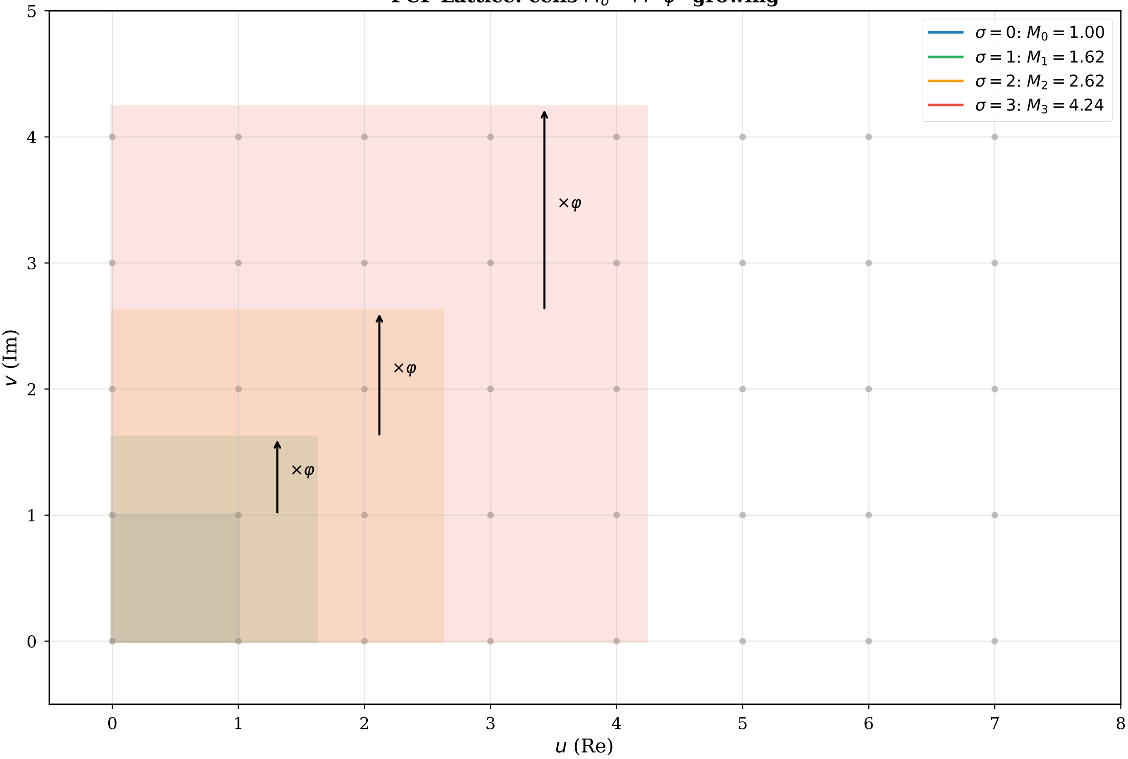
PCF Lattice: cells M_\sigma = M \cdot \varphi^\sigma growing
