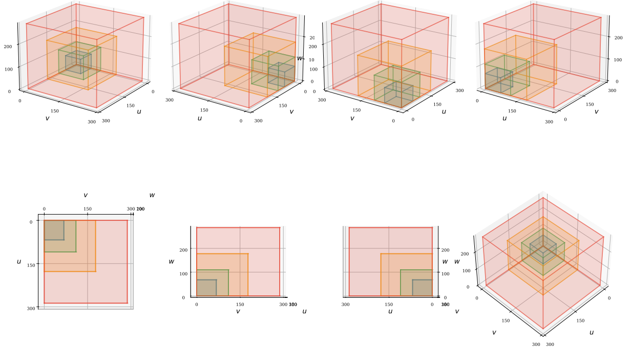
Figure 7. PCF pentadimensional lattice tower with \varphi^\sigma scaling (II). Left: PCF hypercube in eight complementary views — four isometric perspectives (top row) and four orthogonal projections (bottom row) — revealing nested cubic structures scaling as \varphi^\sigma . Right: Full isometric view of the 3D tower with the innermost cell ( \sigma = 0 ) at the origin and successive shells growing by \varphi . The discrete scale dimension \sigma \in \mathbb{Z} parametrizes the pentadimensional structure \mathcal{M}_{\text{PCF}}^5 = M^4 \times S_\sigma^1 .
