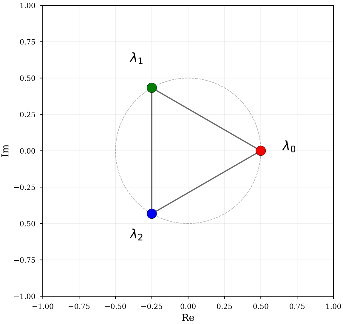
EISENSTEIN: 120^\circ Symmetry
