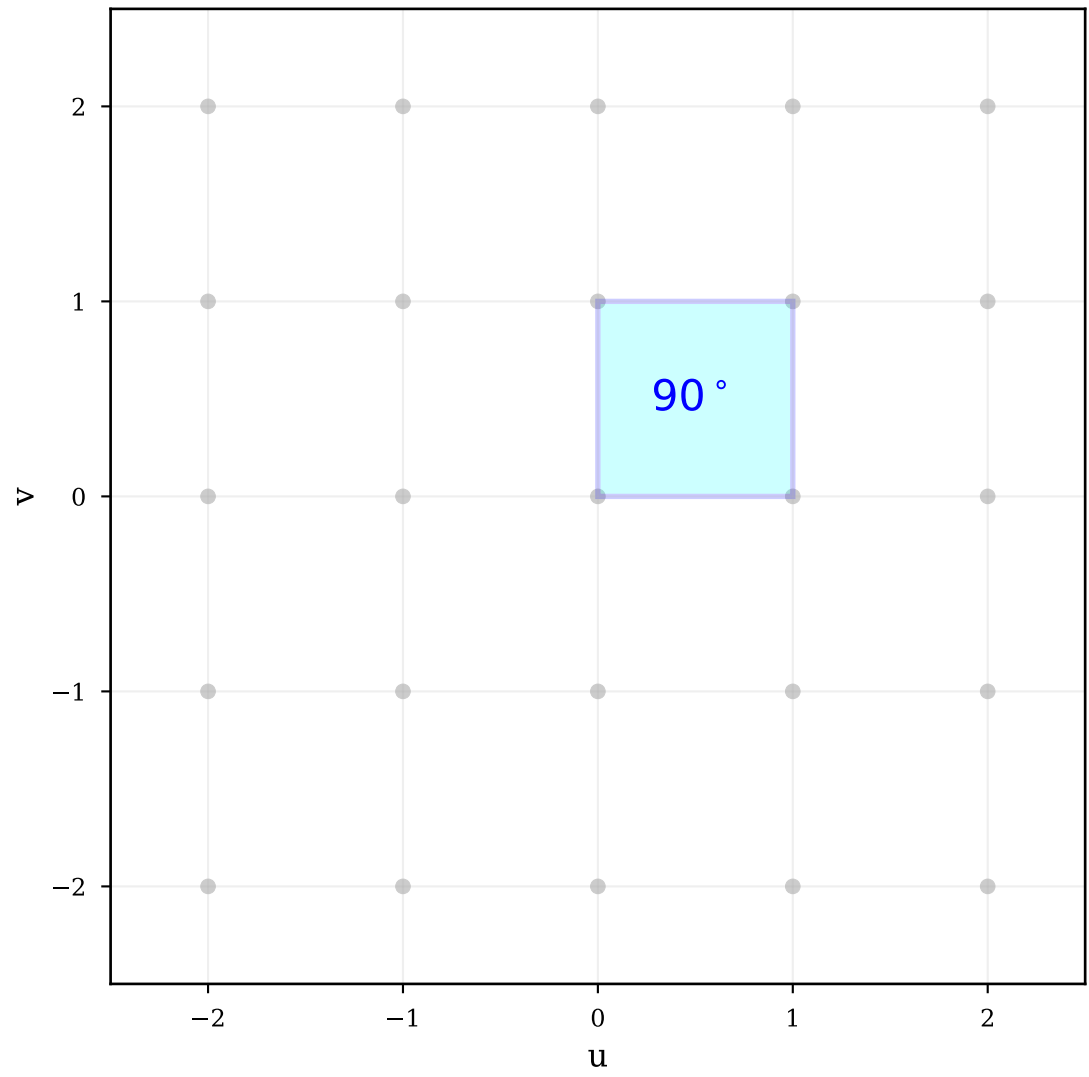
GAUSS: 90^\circ Lattice
