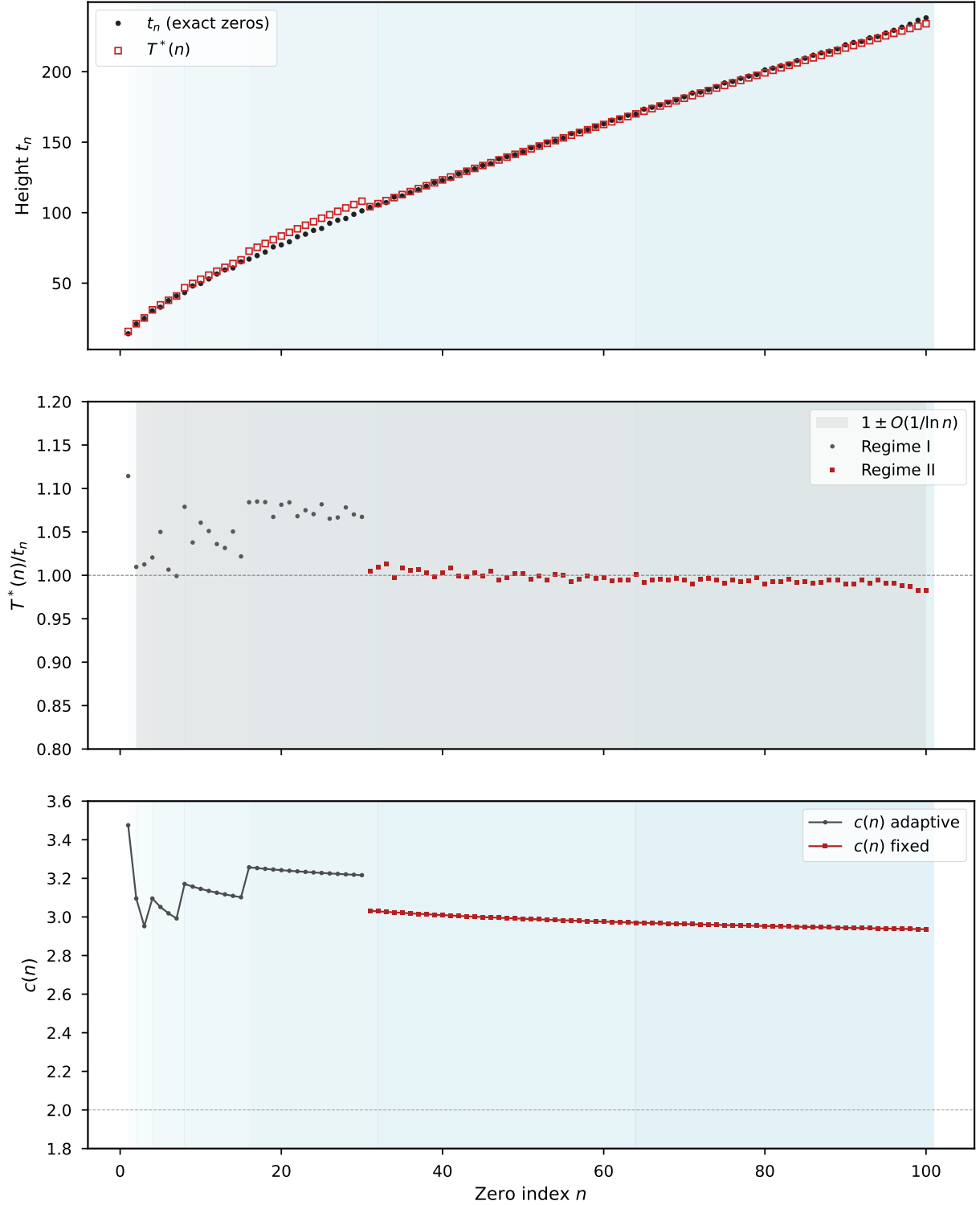
Figure 9. Dual spectral structure and error analytics of T^* . (a) Spectral comparison: Riemann zero heights t_n (black circles) vs. PCF operator eigenvalues T^*(n) (red squares) for the first 100 zeros. Shaded bands denote hypercube generations G_k = [2^k, 2^{k+1}) . (b) Ratio T^*(n)/t_n : showing the adaptive Regime I (gray) and fixed Regime II (red) within the 1 \pm O(1/\ln n) analytical envelope (shaded gray). (c) Structural modulation c(n) : the dual tower structure connecting binary boundaries 2^k and Mersenne primes M_p to the golden expansion \varphi , converging to the spectral sum limit \sigma + \mu = 2 (dashed line).
