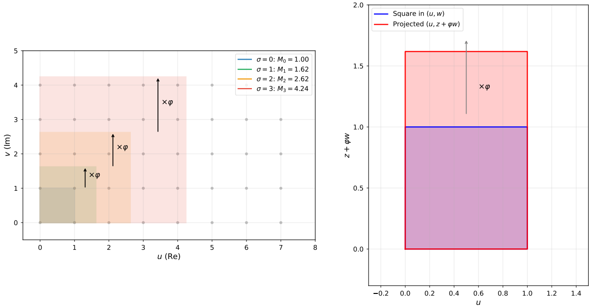
Figure 7. PCF lattice growth and structural projection. Left: Lattice \Lambda_{\text{PCF}} with fundamental cells M_\sigma = M_{\text{PCF}} \cdot \varphi^\sigma at levels \sigma = 0, 1, 2, 3 , showing self-similar growth by factor \varphi between consecutive levels. Right: Golden coupling projection: a square in (u, w) coordinates maps to a rectangle in (u, z + \varphi w) coordinates, with vertical expansion by factor \varphi (Axiom 3).
