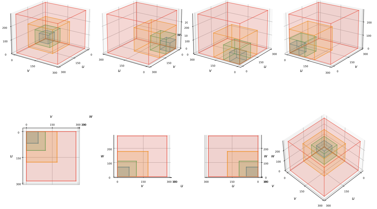
Figure 8. PCF pentadimensional lattice tower with \varphi^\sigma scaling. Top row: PCF hypercube in eight complementary views — four isometric perspectives — revealing nested cubic structures scaling as \varphi^\sigma . Bottom row: Four orthogonal projections revealing the rigid cubic scaffolding. Full isometric view of the 3D tower with the innermost cell ( \sigma = 0 ) at the origin and successive shells growing by \varphi . The discrete scale dimension \sigma \in \mathbb{Z} parametrizes the pentadimensional structure \mathcal{M}_{\text{PCF}}^5 = M^4 \times S_\sigma^1 .
