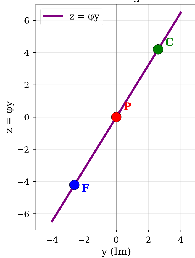
Lateral view: Line z=\phi y Vertices aligned
