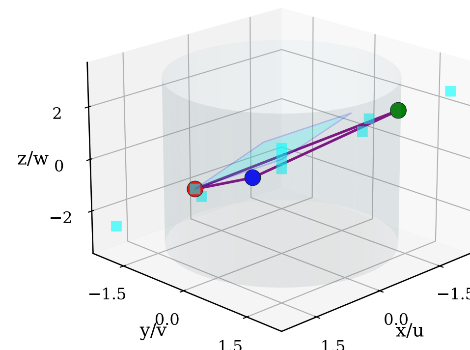
Superposition Triangle in lattice
