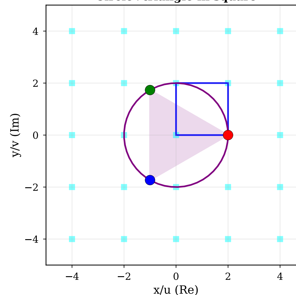
Top view: Superposition Circle+triangle in square
