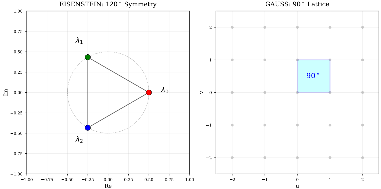
FIGURE 3. Lattice symmetry bridge: Eisenstein to Gauss via \varphi -coupling.
