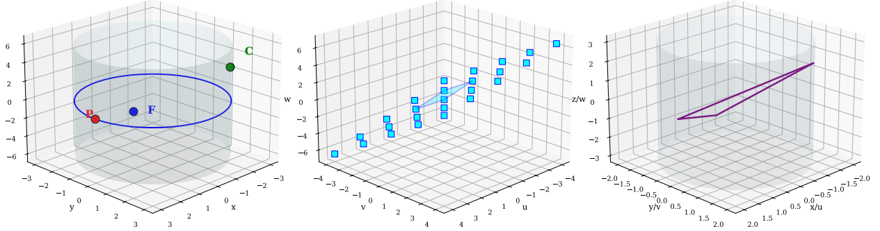
FIGURE 4. Geometric embedding of the tripartite state in the PCF lattice.
