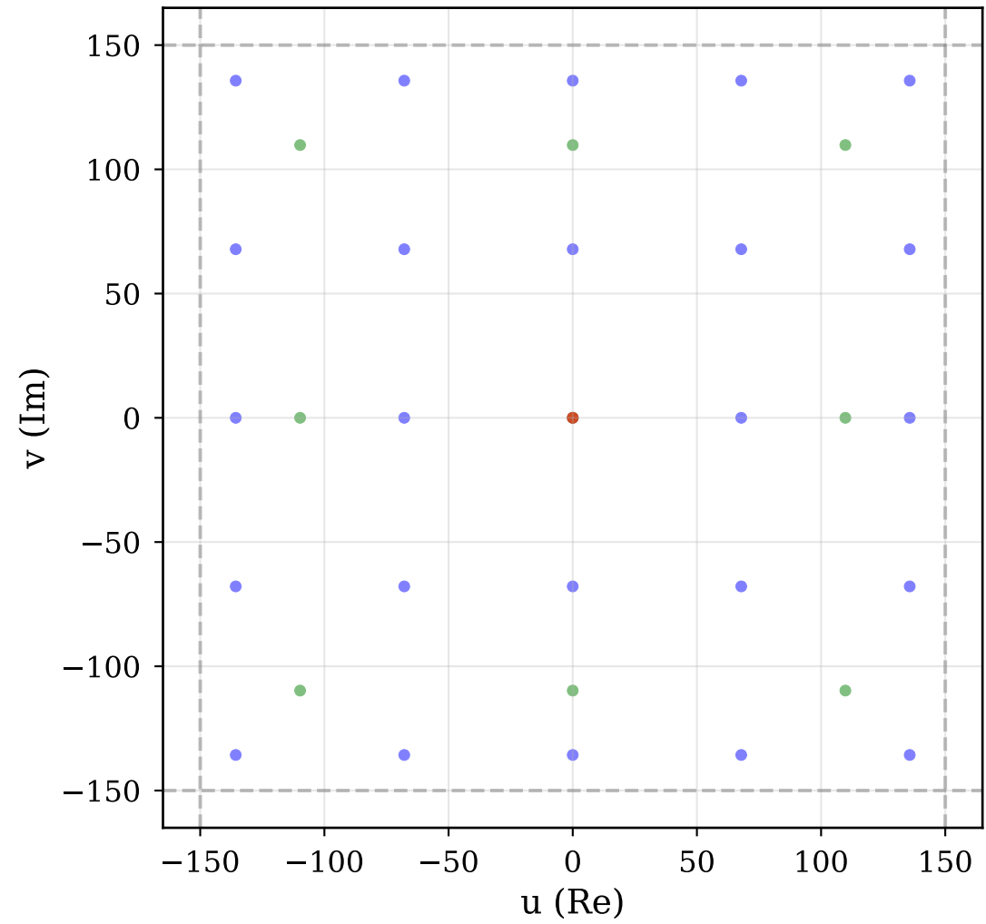
Fixed volume [-150, 150]^2 (lower \sigma = denser)
