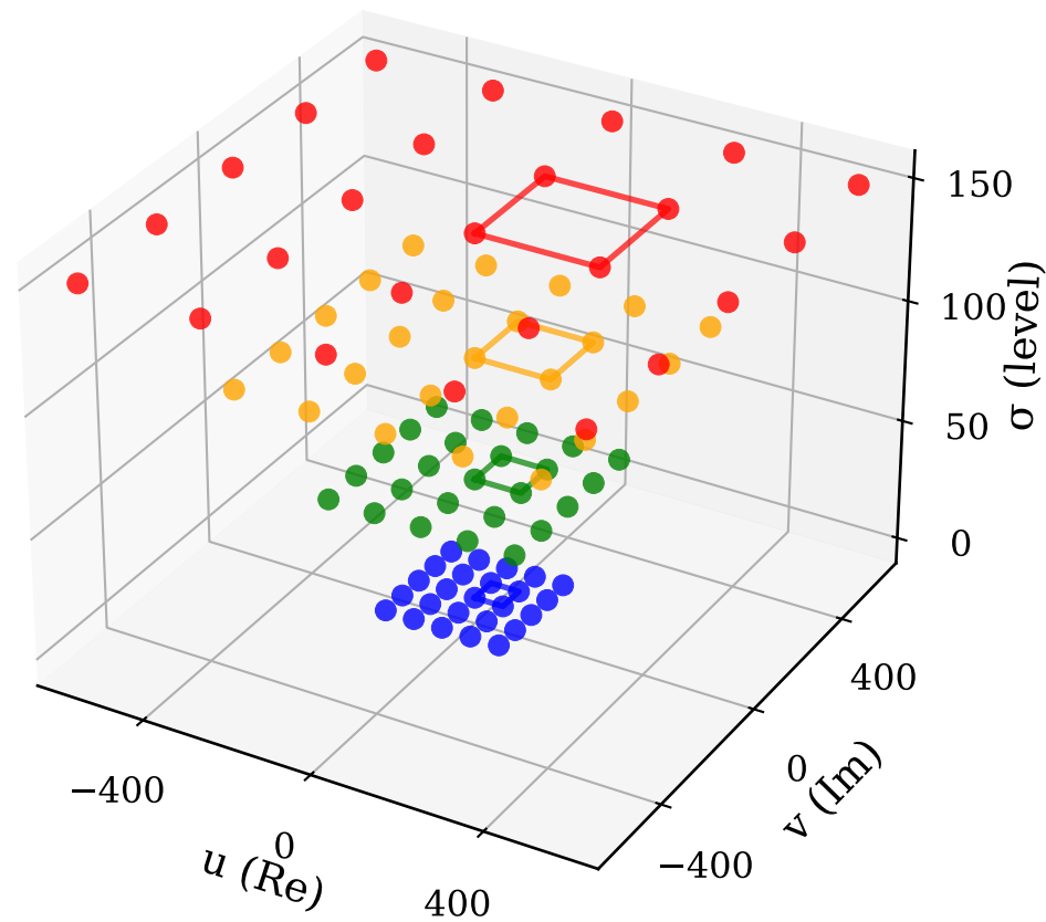
PCF Hypercube (Absolute coordinates)
