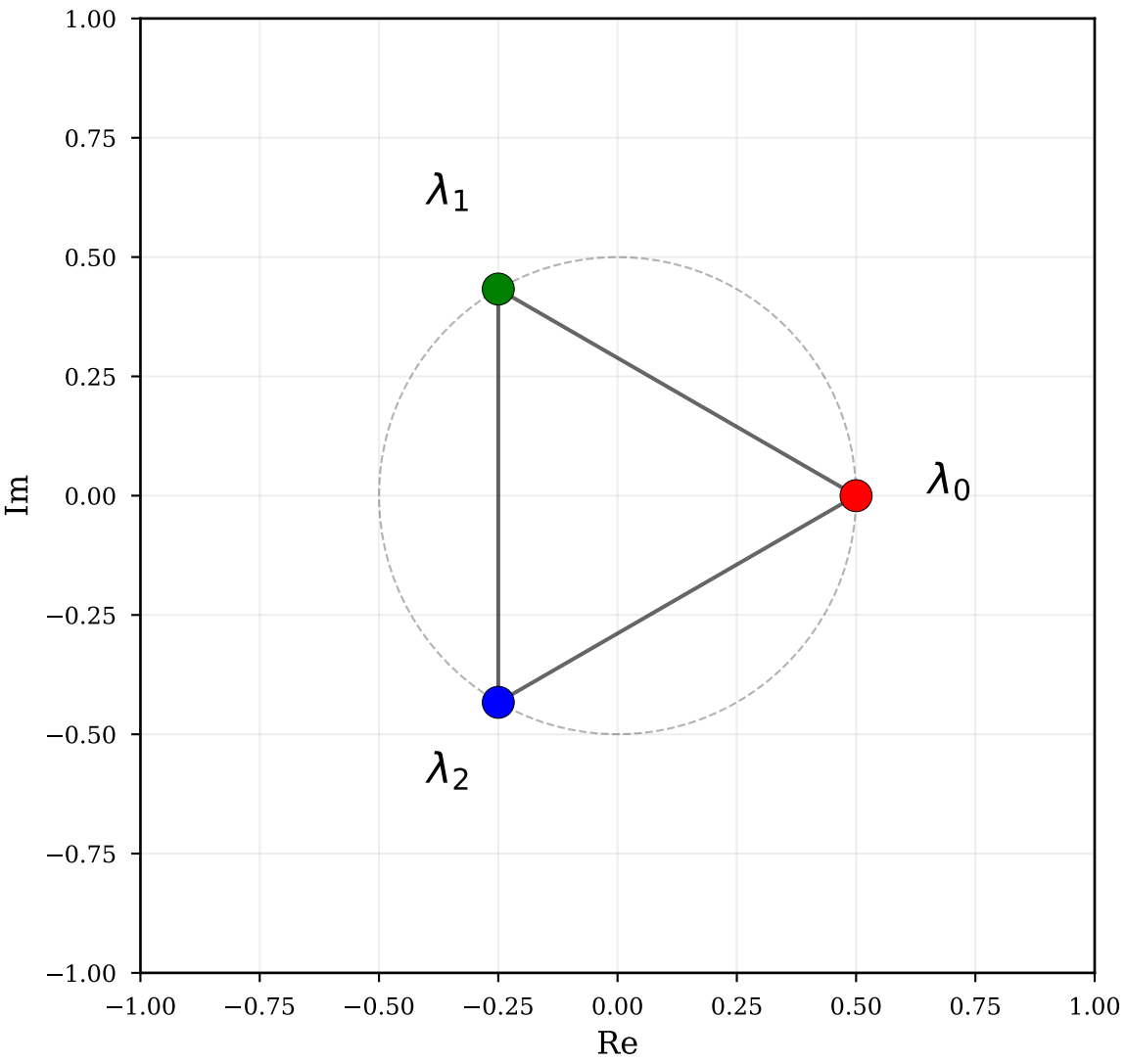
EISENSTEIN: 120° Symmetry
