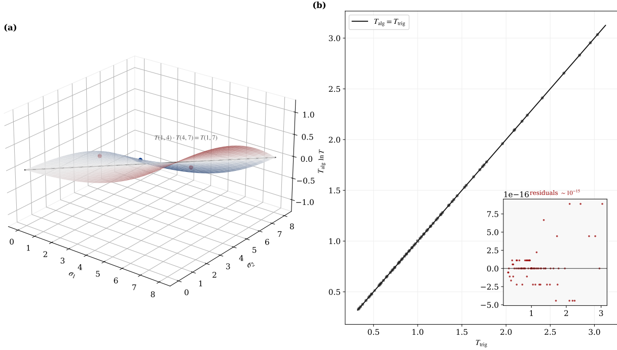
FIGURE 4. ER = EPR from the modulus (Prop. 3.16): (a) the bridge amplitude T(\sigma_1, \sigma_2) as a cocycle, T(1, 4)T(4, 7) = T(1, 7) ; (b) the algebraic and trigonometric forms agree, T_{\text{alg}} = T_{\text{trig}} , to machine precision — which is Corollary 3.17, (3.29), and not a numerical accident.
