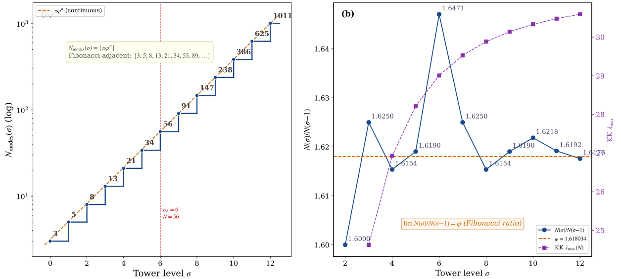
FIGURE 3. The mode tower N_{\text{modes}}(\sigma) = \lfloor \pi\varphi^\sigma \rfloor (3.12): (a) the Fibonacci-adjacent staircase \{3, 5, 8, 13, 21, 34, 56, \dots\} , equal to the Fibonacci values for \sigma \leq 5 and departing at \sigma = 6 where 56 \neq 55 (Remark 3.6); (b) the successive ratio N_{\text{modes}}(\sigma)/N_{\text{modes}}(\sigma-1) \rightarrow \varphi alongside the Kaluza–Klein spectrum.
