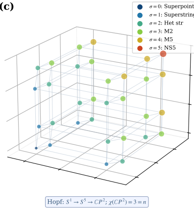
FIGURE 4. AdS_5 funnel z = \varphi^\sigma (3.18) \leftrightarrow the lattice tower \Lambda_\sigma \leftrightarrow the Hamming hypercube H_5 of the M-theory ladder (superpoint \rightarrow NS5); \varphi^\sigma connects all three: (a) the funnel with \ell = 1 , G_N = \frac{1}{2} ; levels bottom-to-top are superpoint ( \sigma=0 ), superstring ( \sigma=1 ), het string ( \sigma=2 ), M2-brane ( \sigma=3 ), M5-brane ( \sigma=4 ), NS5-brane ( \sigma=5 ), 10-brane ( \sigma=6 ); (b) the Eisenstein lattice \Lambda_\sigma = \varphi^\sigma \Lambda_{PCF} in \mathbb{C} with concentric \varphi -rings; (c) the Hamming cube H_5 = \{0,1\}^5 coloured by Hamming weight = H-S level.
