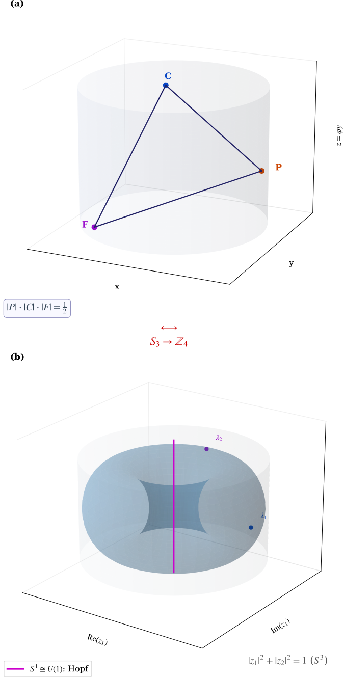
FIGURE 8. From \varphi^2 = \varphi + 1 : (a) the cylinder C_0 with P, C, F at 120^\circ ( \|P\| \|C\| \|F\| = \frac{1}{2} ) closes to (b) the torus T_{\text{PCF}}^2 = \mathbb{C}/\Lambda , \tau = i ( |z_1|^2 + |z_2|^2 = \frac{1}{4} + \frac{3}{4} = 1 , the S^3 constraint), whose Clifford embedding T^2 \hookrightarrow S^3 and Hopf fibre give the gauge factors \text{SU}(3) \times \text{SU}(2) \times \text{U}(1) of App. A.3.
