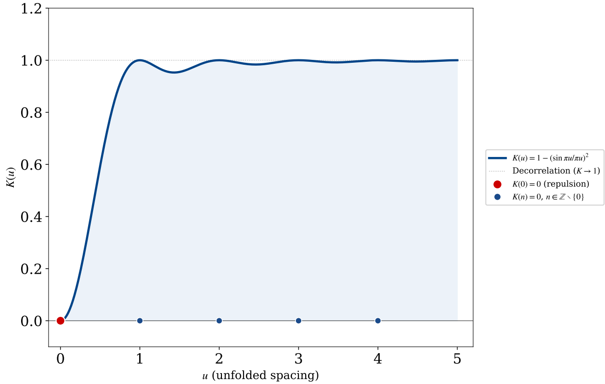
FIGURE 2. The GUE pair-correlation kernel K(u) = 1 - (\sin \pi u / \pi u)^2 of Def. 2.87. The red point at K(0)=0 is level repulsion—the suppression of small spacings that Def. 2.81 measures. Blue points mark K(n)=0 for n \in \mathbb{Z} \setminus \{0\} (no long-range correlation). The kernel tends to 1 for large u (decorrelation).
