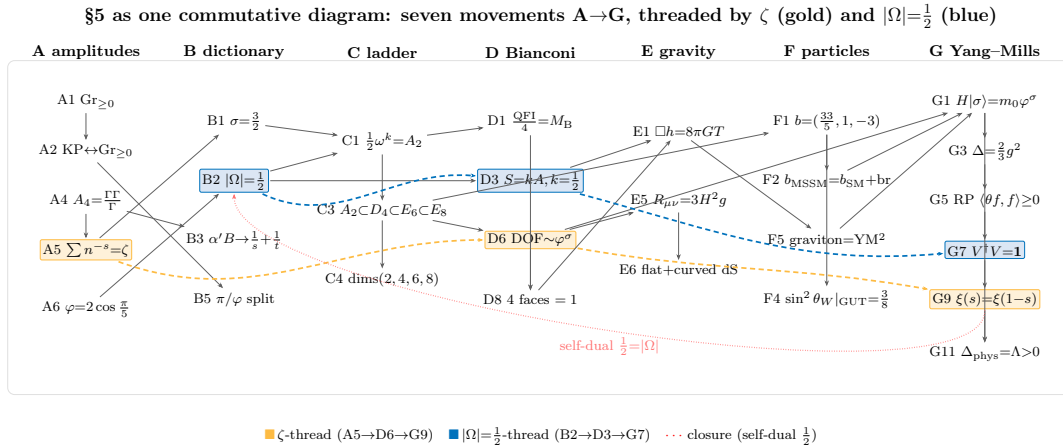
FIGURE 14. Commutative diagram of §5: its demonstrative skeleton across the seven movements (A amplitudes, B dictionary, C ladder, D Bianconi, E gravity, F particles/SUSY, G Yang–Mills), threaded by \zeta (gold) and |\Omega| = \frac{1}{2} (blue), closing on the self-dual \frac{1}{2} .
