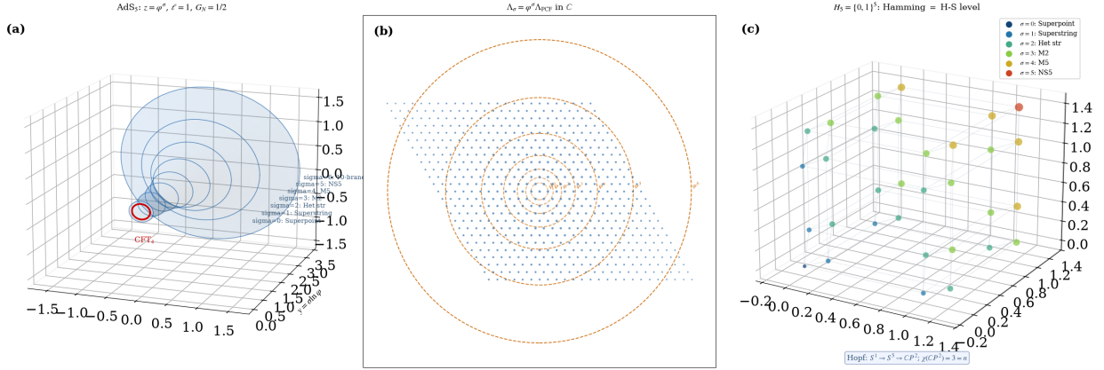
Figure 3: \text{AdS}_5 funnel z = \varphi^\sigma (50) \leftrightarrow the lattice tower \Lambda_\sigma \leftrightarrow the Hamming hypercube H_5 of the M-theory ladder (superpoint \rightarrow NS5); \varphi^\sigma connects all three.
