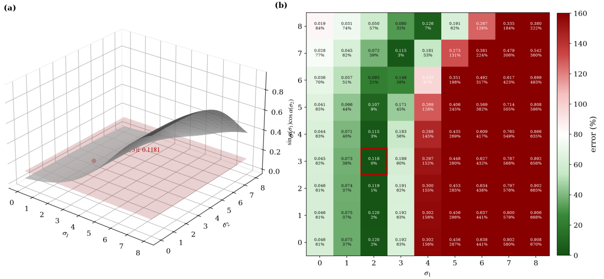
Figure 1: The spectral angle \alpha(\sigma) = \arctan(\varepsilon_0 \varphi^\sigma) : (a) the surface \sin \alpha(\sigma_1) \cos \alpha(\sigma_2) ; (b) the error map, vanishing only at (\sigma_1, \sigma_2) = (2, 3) (boxed) — the unique pair compatible with the forced invariants (40).
