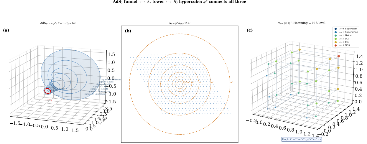
FIGURE 3. AdS 5 funnel z = \varphi^\sigma (3.16) \leftrightarrow the lattice tower \Lambda_\sigma \leftrightarrow the Hamming hypercube H_5 of the M-theory ladder (superpoint \rightarrow NS5); \varphi^\sigma connects all three.
