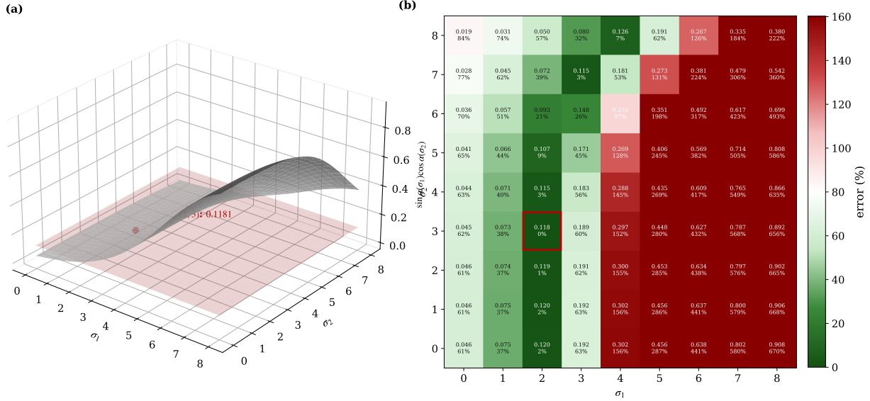
FIGURE 7. (a) The spectral-angle surface \sin \alpha(\sigma_1) \cos \alpha(\sigma_2) of (3.8), whose tangent climbs at the rate \varphi of (3.7) of §3.2; the marked point is the level pair (\sigma_G, \sigma_{EM}) = (2, 3) of (4.26). (b) How many of the four constraints of Proposition 4.20 each integer triple (\sigma_G, \sigma_{EM}, \sigma_\Lambda) satisfies: the boxed (2, 3, 6) is the only one satisfying all four, every other triple failing at least one. No fitted quantity enters either panel.
