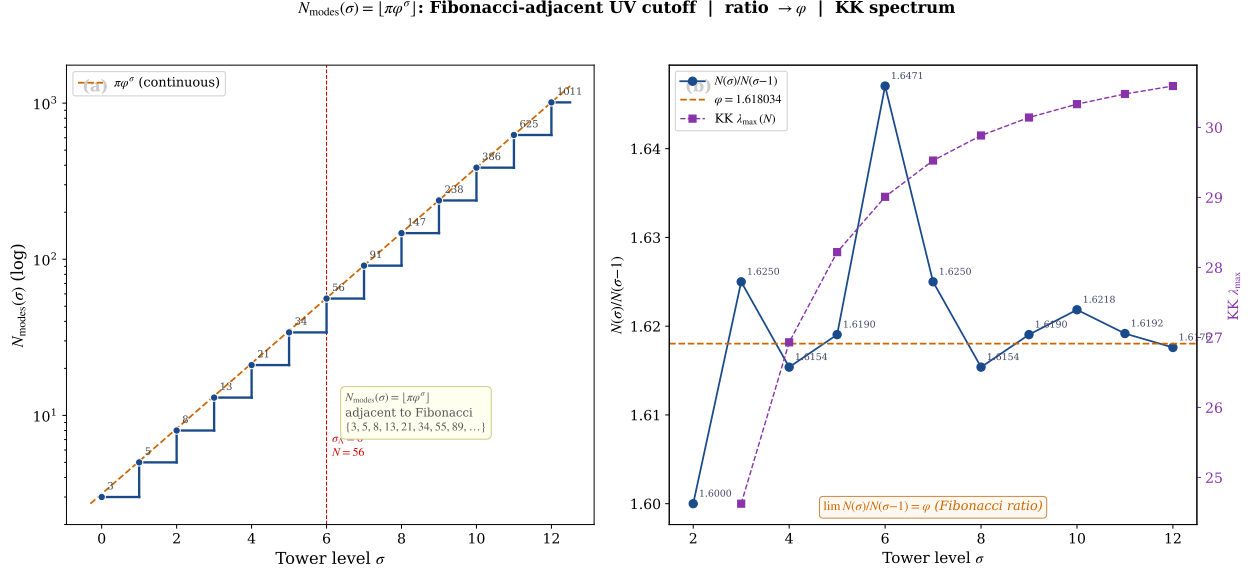
FIGURE 1. The mode tower N_{\text{modes}}(\sigma) = \lfloor \pi \varphi^\sigma \rfloor (3.12): (a) the Fibonacci-adjacent staircase \{3, 5, 8, 13, 21, 34, 56, \dots\} , equal to the Fibonacci values for \sigma \leq 5 and departing at \sigma = 6 where 56 \neq 55 (Remark 3.6); (b) the successive ratio N_{\text{modes}}(\sigma)/N_{\text{modes}}(\sigma-1) \rightarrow \varphi alongside the Kaluza–Klein spectrum.
