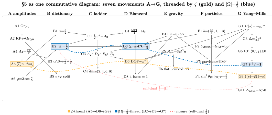
FIGURE 12. Commutative diagram of §5: its demonstrative skeleton across the seven movements (A amplitudes, B dictionary, C ladder, D Bianconi, E gravity, F particles/SUSY, G Yang–Mills), threaded by \zeta (gold) and |\Omega| = \frac{1}{2} (blue), closing on the self-dual \frac{1}{2} .
