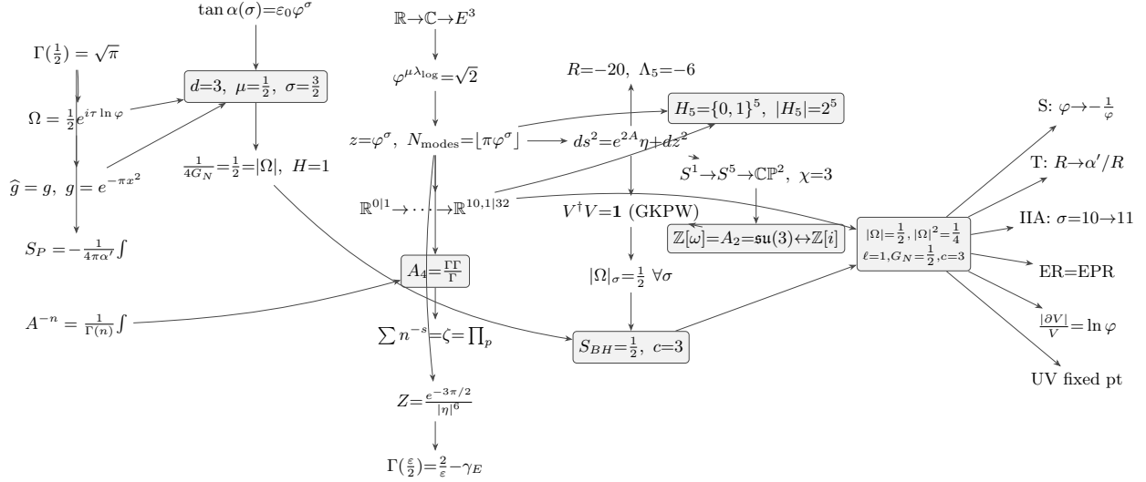
FIGURE 5. Commutative spine of §3 (P1→P20): the thirty-one nodes carrying the twenty steps, arranged by subsection (the object, §3.1; the meta-invariant, §3.2; the tower and amplitudes, §3.3; AdS/CFT per level, §3.4; the duality web, §3.5), with the thirty-four demonstrative arrows. Shaded nodes are the six apices, where two or more independent chains converge on the same value; the forced invariants d=3, \mu=\frac{1}{2}, \sigma=\frac{3}{2} , with three incoming routes, are the maximal one. Seeded by the arithmetic of K = \mathbb{Q}(\sqrt{5}) in §2; mathematical, physical and conceptual layers coincide on one diagram.
