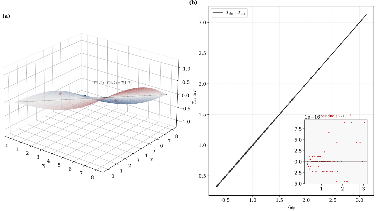
FIGURE 4. ER = EPR from the modulus (Prop. 3.16): (a) the bridge amplitude T(\sigma_1, \sigma_2) as a cocycle, T(1, 4)T(4, 7) = T(1, 7) ; (b) the algebraic and trigonometric forms agree, T_{\text{alg}} = T_{\text{trig}} , to machine precision — which is Corollary 3.17, (3.29), and not a numerical accident.
