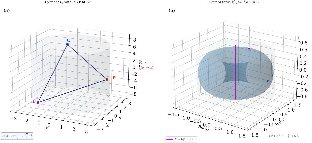
FIGURE 6. From \varphi^2 = \varphi + 1 : the cylinder C_0 with P, C, F at 120^\circ ( \|P\| \|C\| \|F\| = \frac{1}{2} ) closes to the torus T_{\text{PCF}}^2 = \mathbb{C}/\Lambda , \tau = i , whose Clifford embedding T^2 \hookrightarrow S^3 and Hopf fibre give the gauge factors \text{SU}(3) \times \text{SU}(2) \times \text{U}(1) of App. A.3.
