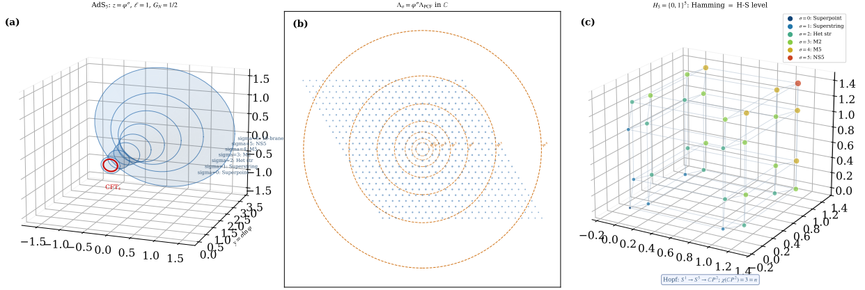
FIGURE 2. AdS 5 funnel z = \varphi^\sigma (3.18) \leftrightarrow the lattice tower \Lambda_\sigma \leftrightarrow the Hamming hypercube H_5 of the M-theory ladder (superpoint \rightarrow NS5); \varphi^\sigma connects all three.
