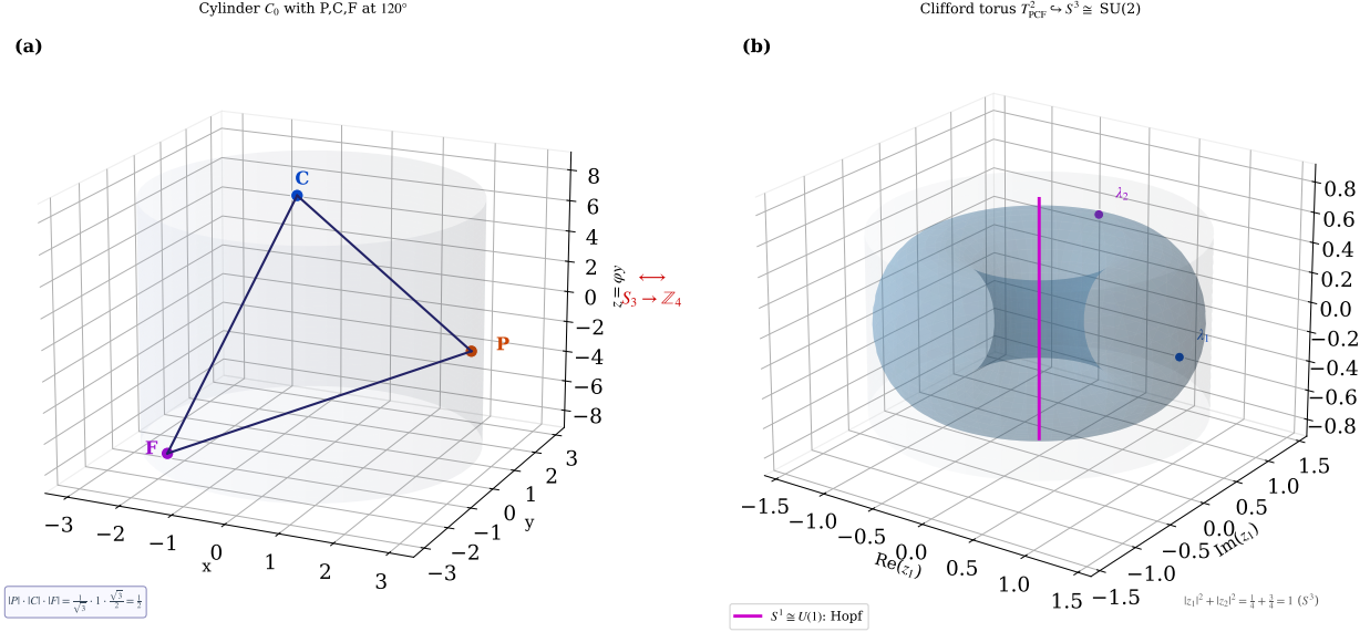
FIGURE 6. From \varphi^2 = \varphi + 1 : the cylinder C_0 with P, C, F at 120^\circ ( \|P\| \|C\| \|F\| = \frac{1}{2} ) closes to the torus T_{\text{PCF}}^2 = \mathbb{C}/\Lambda , \tau = i , whose Clifford embedding T^2 \hookrightarrow S^3 and Hopf fibre give the gauge factors \text{SU}(3) \times \text{SU}(2) \times \text{U}(1) of App. A.3.
