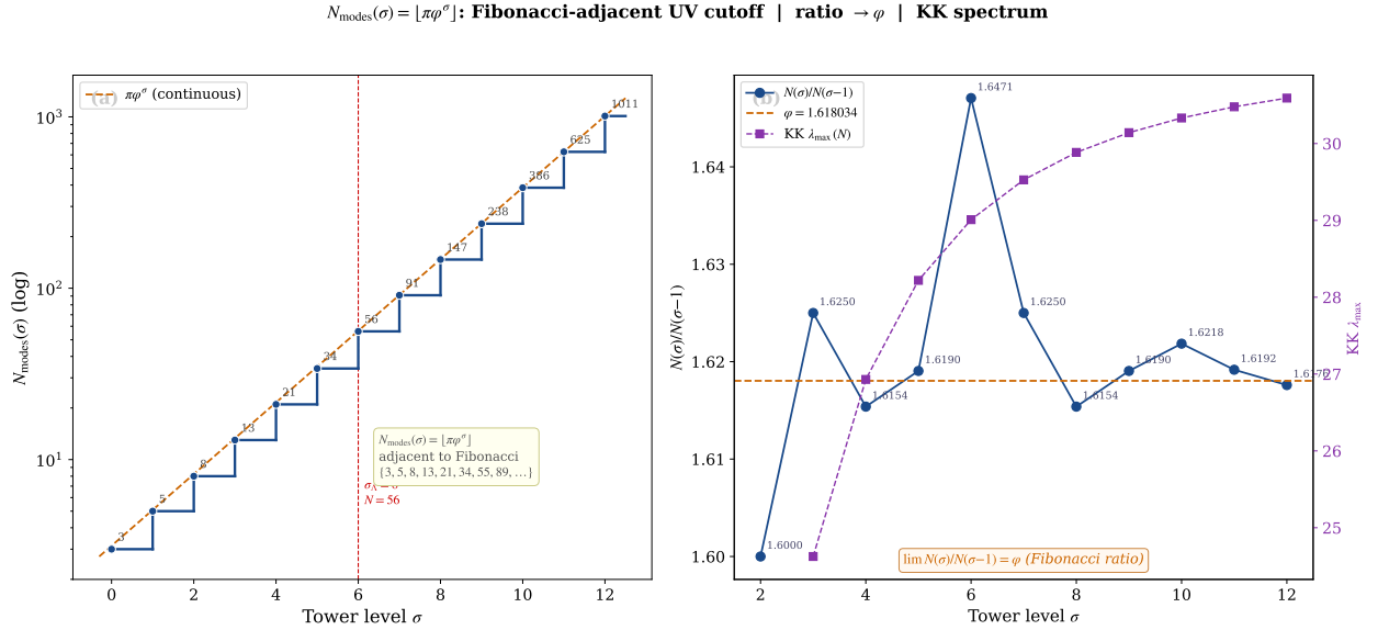
FIGURE 1. The mode tower N_{\text{modes}}(\sigma) = \lfloor \pi\varphi^\sigma \rfloor (3.12): (a) the Fibonacci-adjacent staircase \{3, 5, 8, 13, 21, 34, 56, \dots\} , equal to the Fibonacci values for \sigma \leq 5 and departing at \sigma = 6 where 56 \neq 55 (Remark 3.6); (b) the successive ratio N_{\text{modes}}(\sigma)/N_{\text{modes}}(\sigma-1) \rightarrow \varphi alongside the Kaluza–Klein spectrum.
