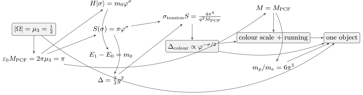
FIGURE 10. Commutative spine of §5 (operators, welded tension, colour): the same microstate \Omega , |\Omega| = \frac{1}{2} , propagates through the scale operator and its gap, the welded tension, the colour scale and running, and the proton placement 6\pi^5 —every arrow uses only earlier nodes, and all converge on the one modulus (Theorem 5.35). Mathematical, string and gauge layers coincide on one diagram; shaded nodes are apices where independent chains meet the same value.
