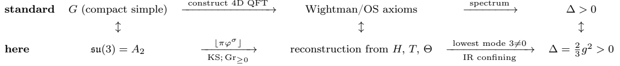
FIGURE 11. The ordering criterion for this section, read as a contrast rather than a claim of identification: the standard route to a gapped four-dimensional gauge theory (top) beside the route taken here (bottom), column by column. Where the standard construction posits a compact simple group, \mathfrak{su}(3) = A_2 is derived from the eigenvalue triangle (Proposition 5.6); where it builds a four-dimensional theory by regularisation, the tower and the positive Grassmannian supply one directly; where it imposes the Wightman/OS axioms, they are recovered from the framework's own operators H , T = e^{-aH} and \Theta (§5.9); and where it asks for a spectral gap, the electric Casimir gives \Delta = \frac{2}{3}g^2 (Theorem 5.21), cutoff-independent by (5.17). Each column is the same requirement met two ways, not a correspondence awaiting proof.
