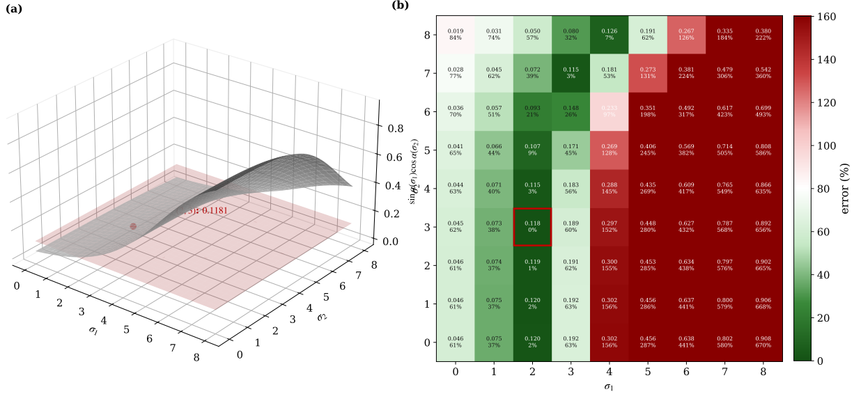
FIGURE 7. (a) The spectral-angle surface \sin \alpha(\sigma_1) \cos \alpha(\sigma_2) of (3.8), whose tangent climbs at the rate \varphi of (3.7) of §3.2; the marked point is the level pair (\sigma_G, \sigma_{EM}) = (2, 3) of (4.26). (b) How many of the four constraints of Proposition 4.20 each integer triple (\sigma_G, \sigma_{EM}, \sigma_\Lambda) satisfies: the boxed (2, 3, 6) is the only one satisfying all four, every other triple failing at least one. No fitted quantity enters either panel.
