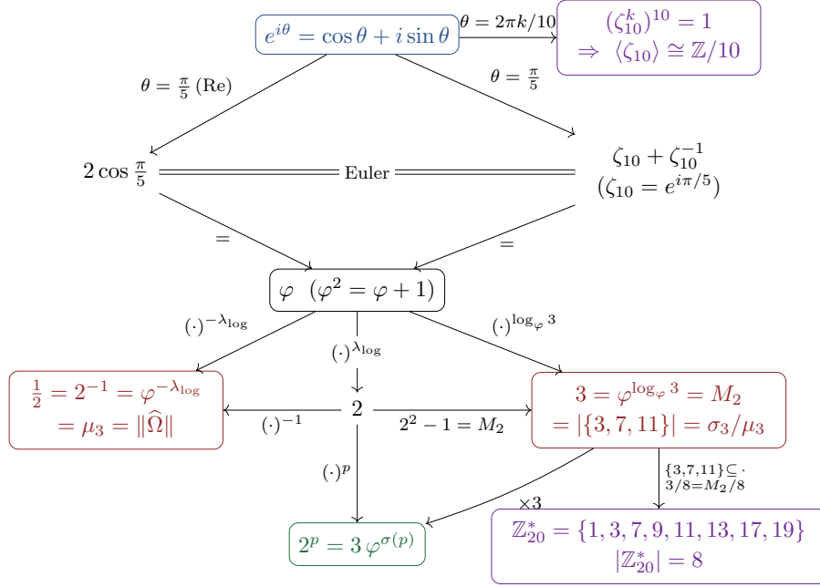
FIGURE 1. The twelve simultaneous identities of Theorem 1.1 (clauses (i)–(xii)), together with the reciprocal turn \varphi^{-\lambda_{\log}} = \frac{1}{2} of Section 5, as a single commutative diagram. Every directed path commutes to the universal identity 3 \varphi^{\sigma(p)} = 2^p (green) and to the reciprocal turn \frac{1}{2} = \varphi^{-\lambda_{\log}} (red, left); the factor 3 = M_2 and the half each appear as a convergence of several identifications under the single algebraic object \varphi .
