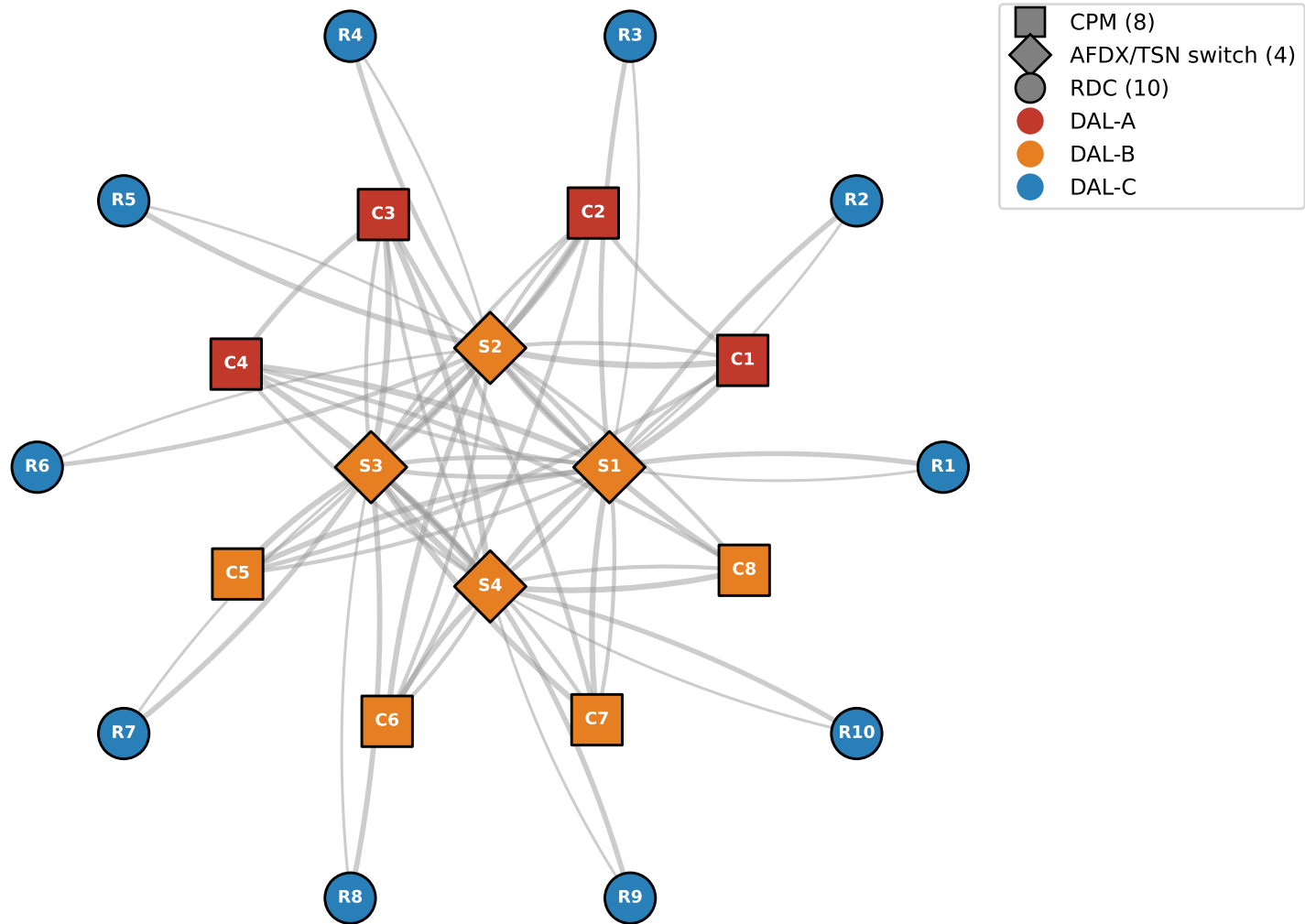
Figure 1. Synthetic 22-node IMA topology (edge thickness \propto dependency weight a_{ij} )
