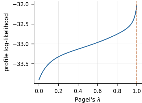
(c) \hat{\lambda} = 1.00 , Blomberg's K = 0.52
