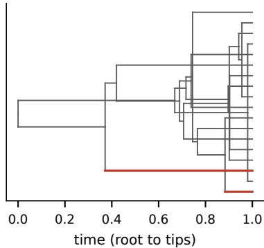
(a) random ultrametric tree
