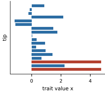
(b) BM trait with induced convergence C_1 = 1.00 (red tips)
