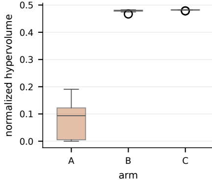
(c) HV over 10 replicates
