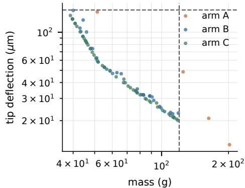
(a) final populations, replicate 0
