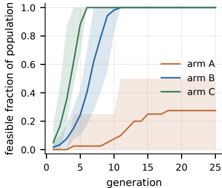
(b) constraint satisfaction
