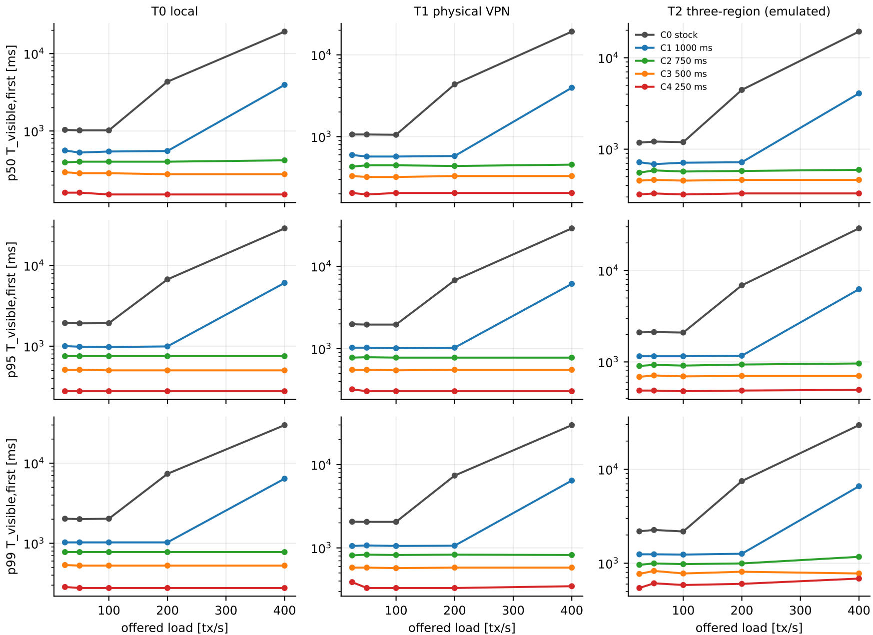
Fig. 5. User-visible latency against offered load
