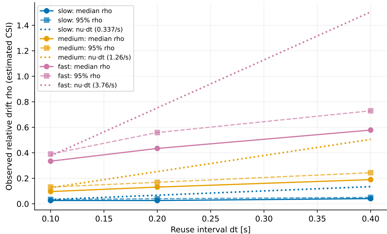
Drift calibration over 1 calibration seeds; linear proxy nu at q=0.95
